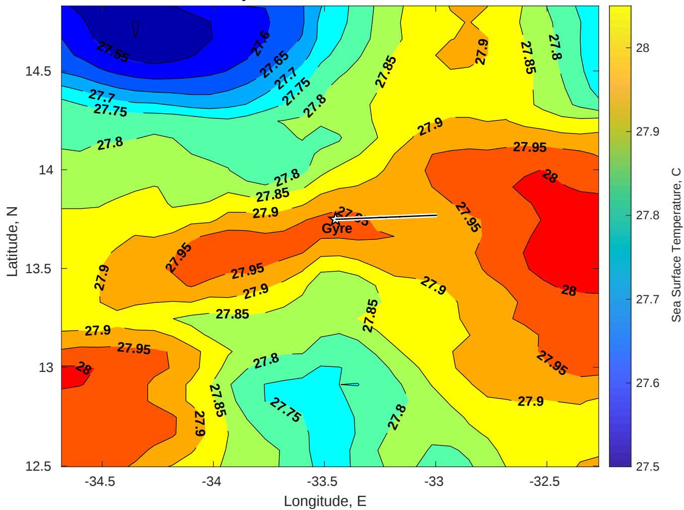
SST for Gyre at 10-Oct-2025 00:00:00
