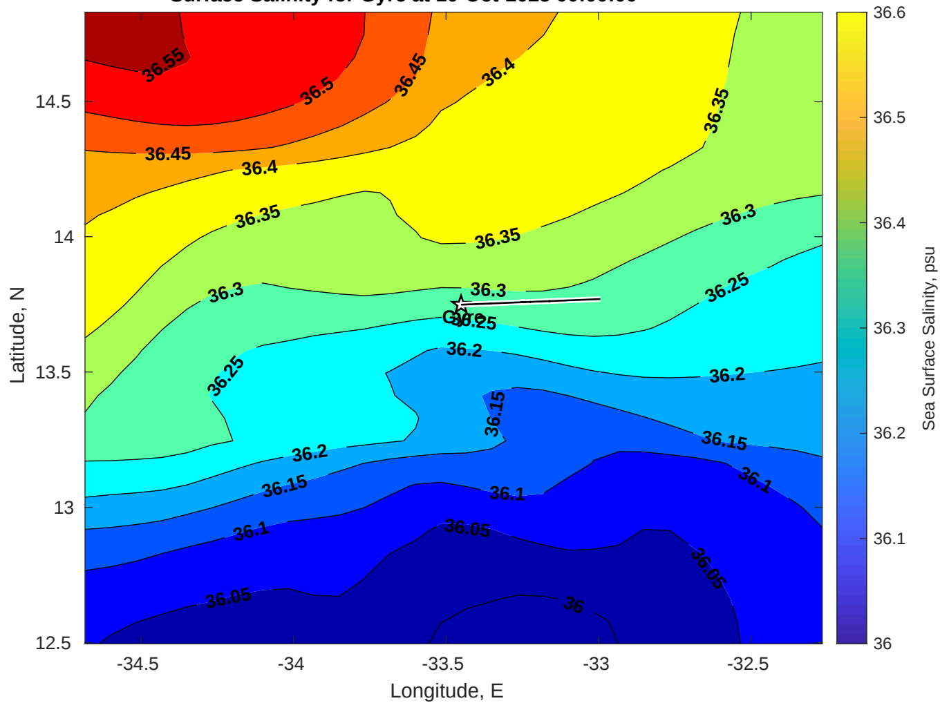
Surface Salinity for Gyre at 10-Oct-2025 00:00:00
