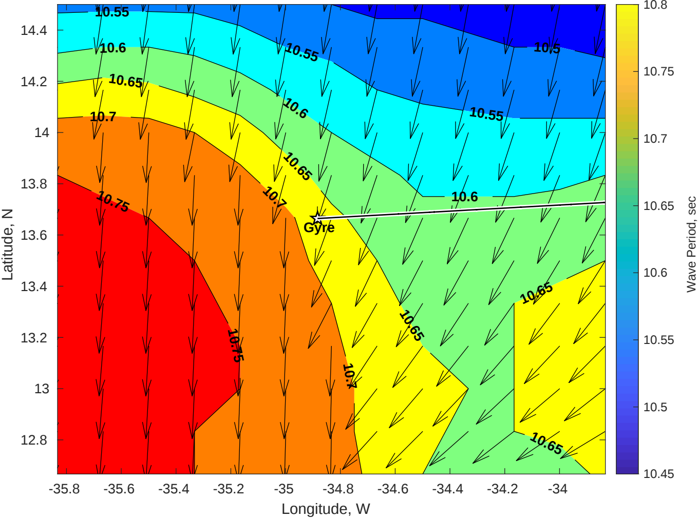
Wave Period (sec) for Gyre at 11-Oct-2025 09:00:00
