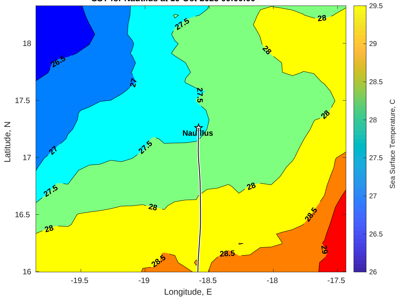
SST for Nautilus at 10-Oct-2025 00:00:00
