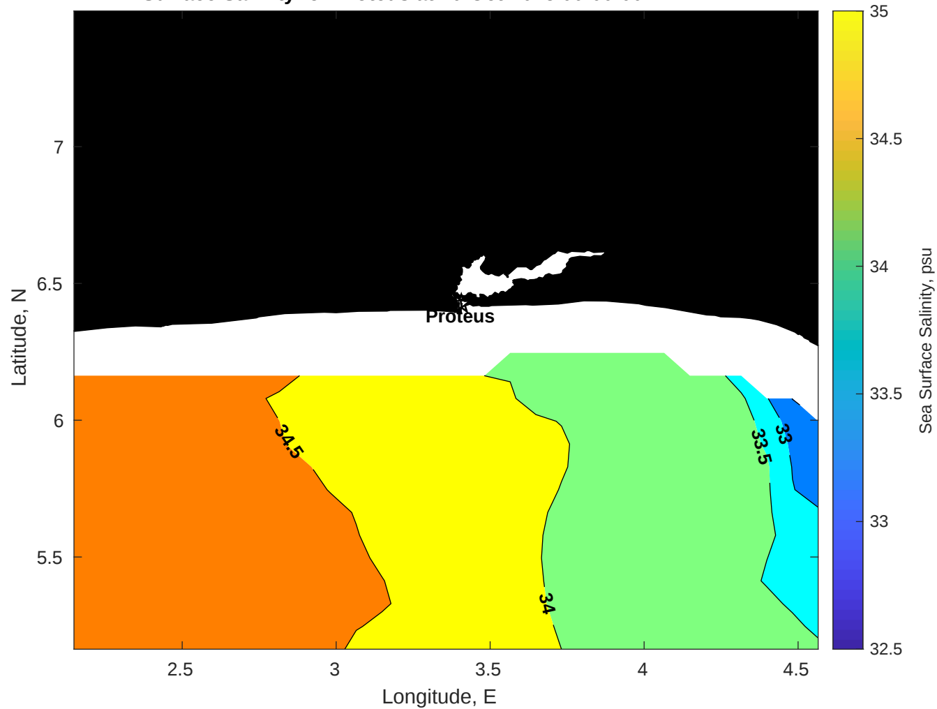
Surface Salinity for Proteus at 10-Oct-2025 00:00:00
