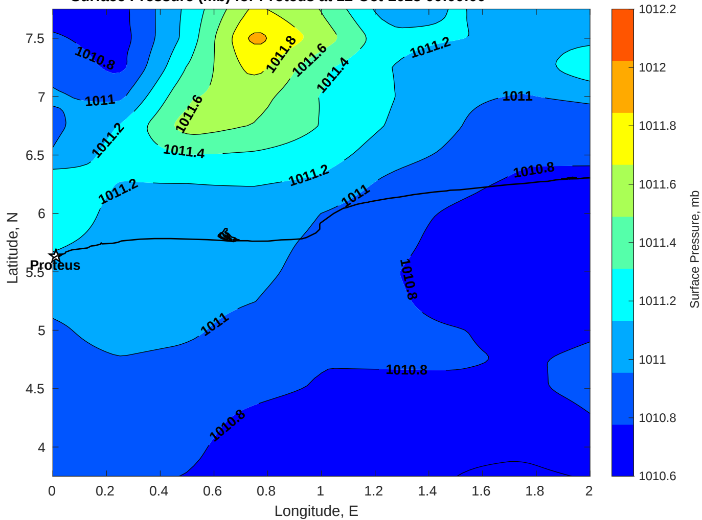
Surface Pressure (mb) for Proteus at 12-Oct-2025 00:00:00
