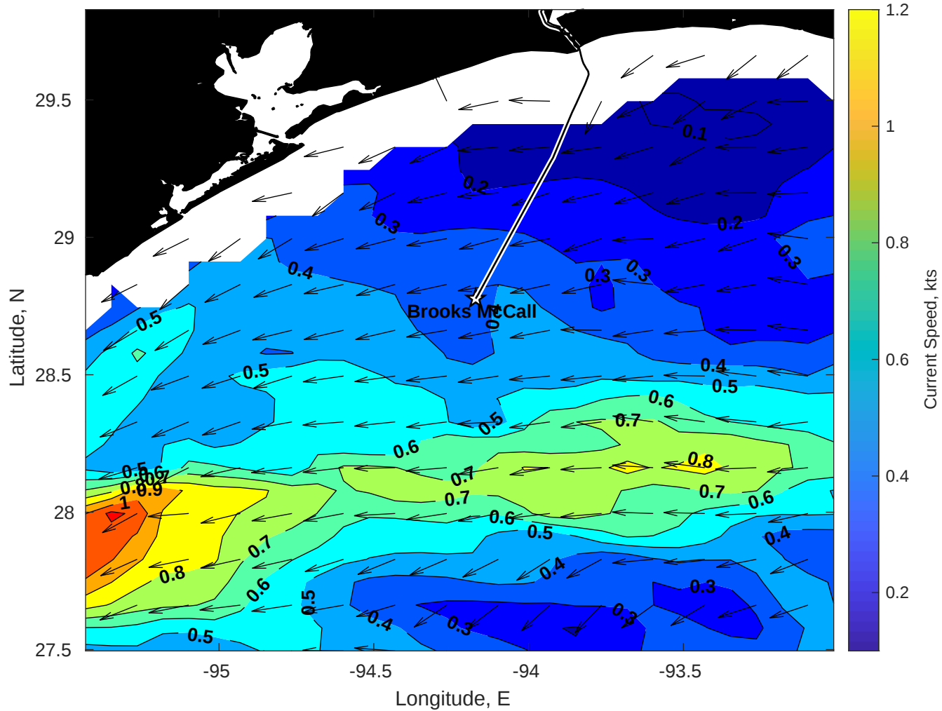
Surface Currents for Brooks McCall at 11-Oct-2025 00:00:00
