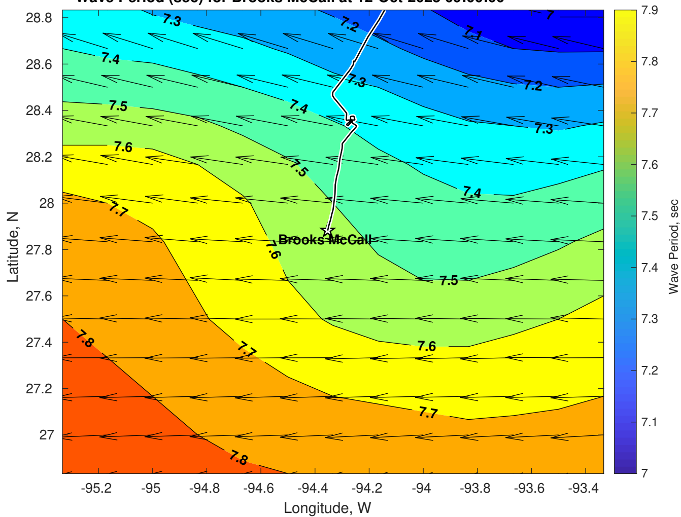
Wave Period (sec) for Brooks McCall at 12-Oct-2025 09:00:00
