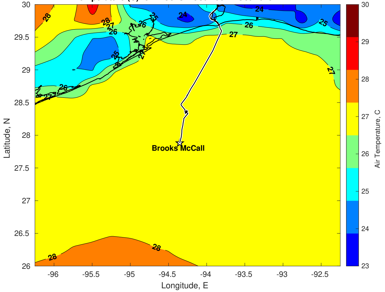
Air Temperature (C) for Brooks McCall at 12-Oct-2025
