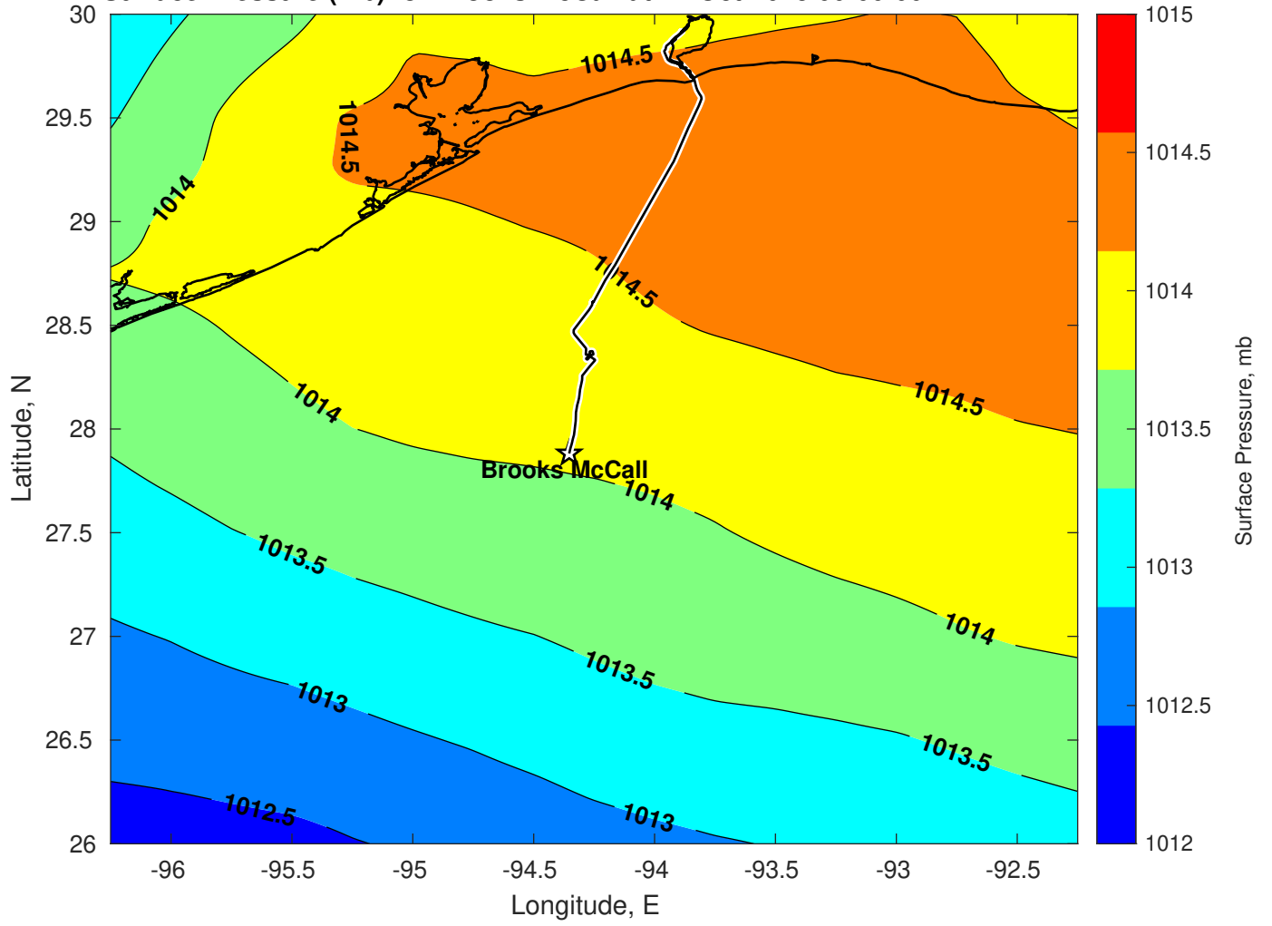
Surface Pressure (mb) for Brooks McCall at 14-Oct-2025 00:00:00
