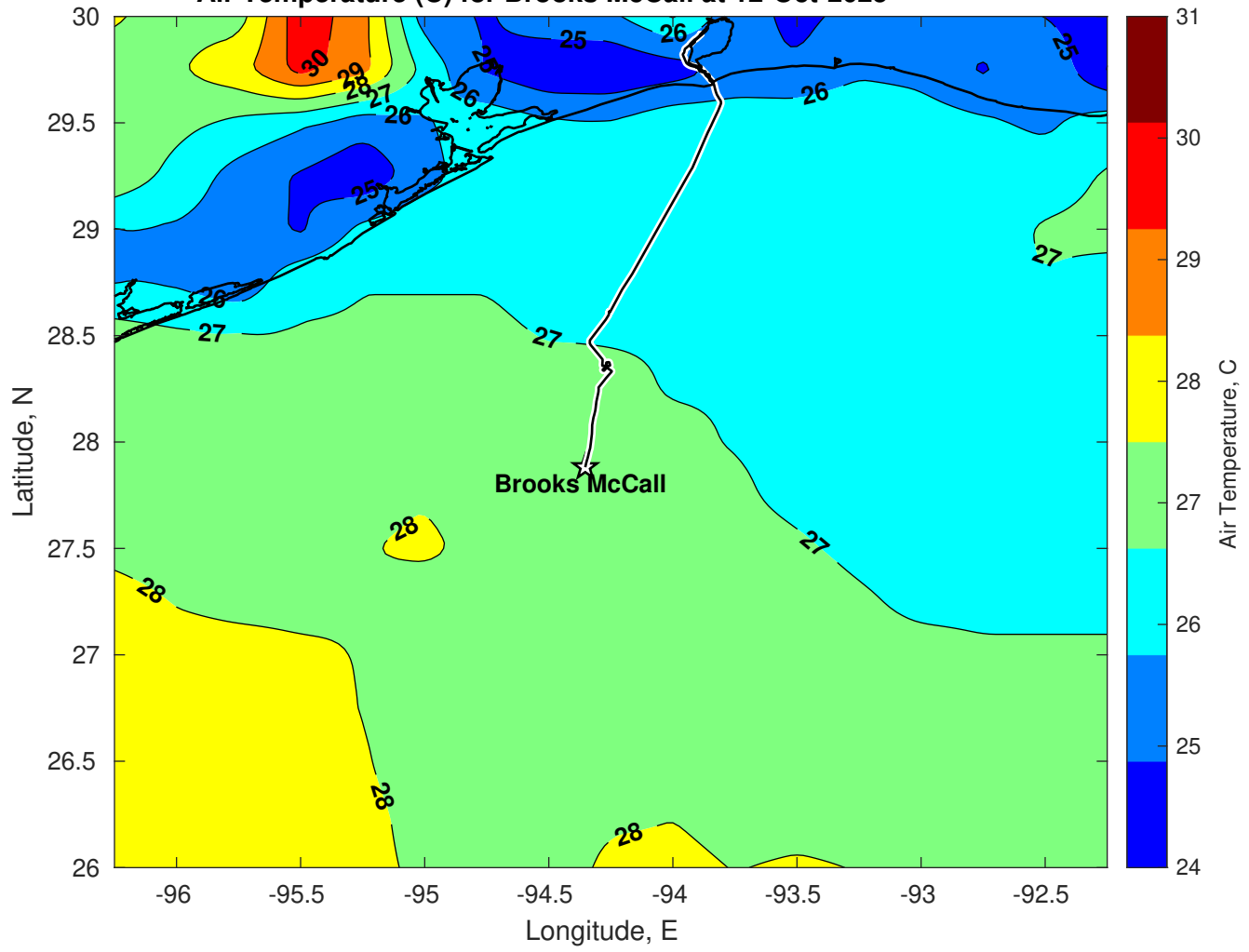
Air Temperature (C) for Brooks McCall at 12-Oct-2025
