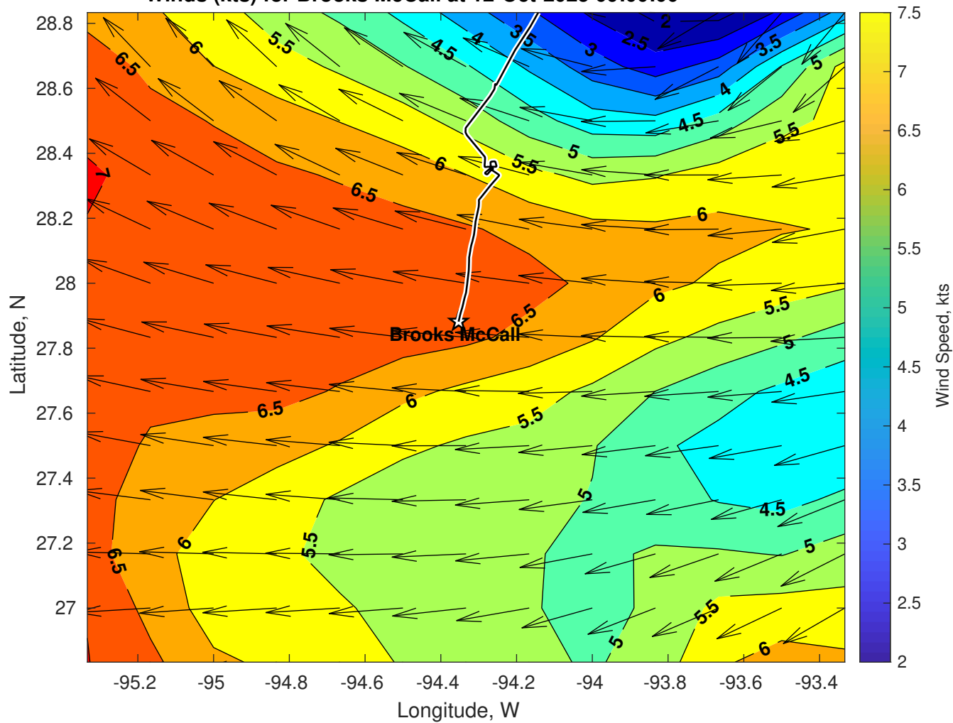
Winds (kts) for Brooks McCall at 12-Oct-2025 09:00:00
