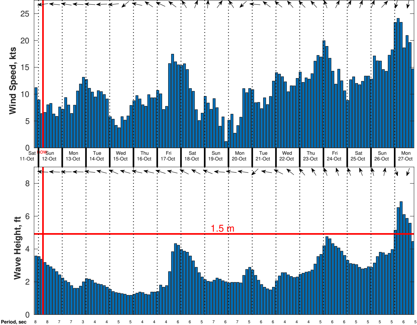
Wind & Wave Forecast for Brooks McCall from 11-Oct-2025 20:00:00 to 27-Oct-2025 20:00:00
