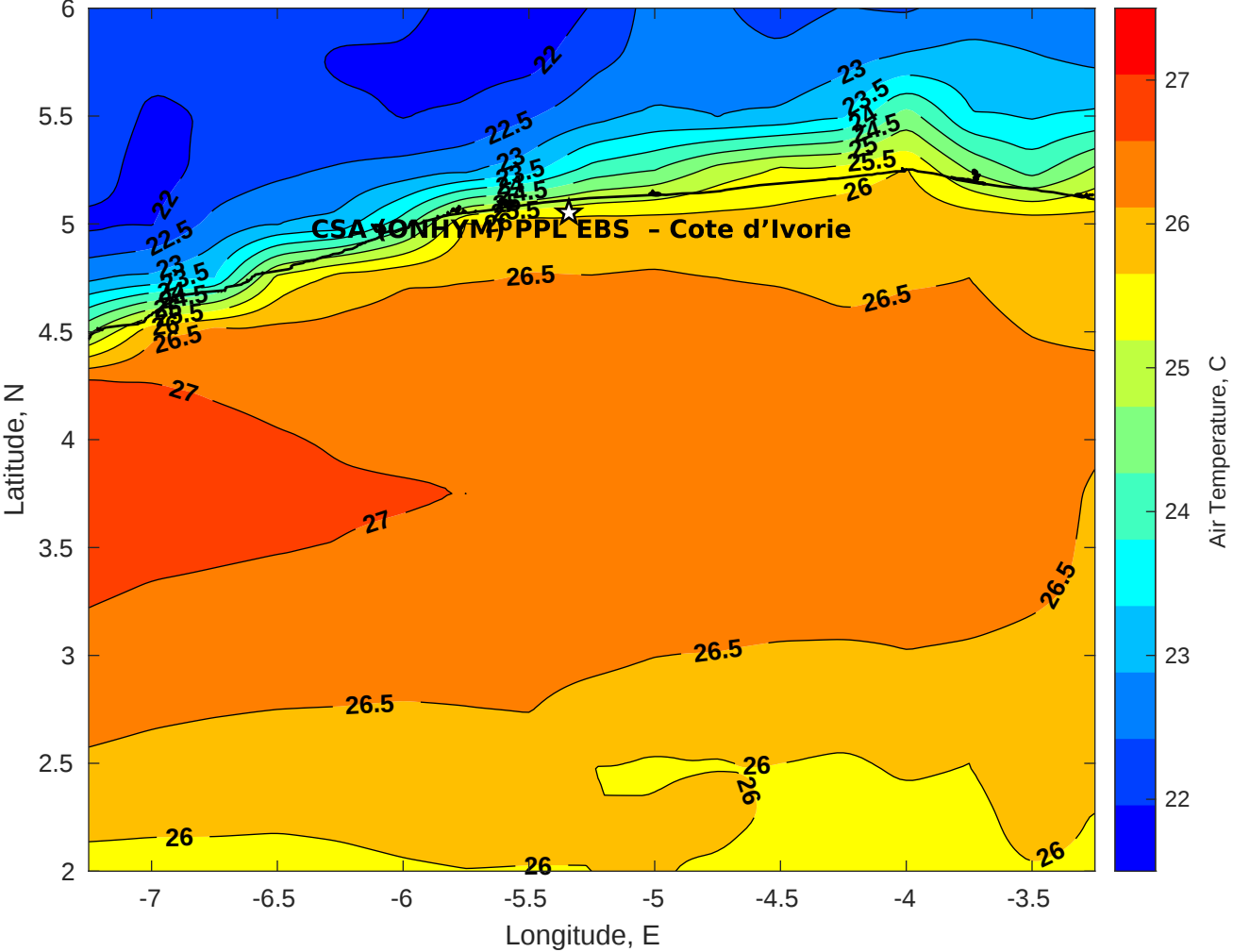
Air Temperature (C) for CSA (ONHYM) PPL EBS - Cote d'Ivoire at 12-Oct-2025
