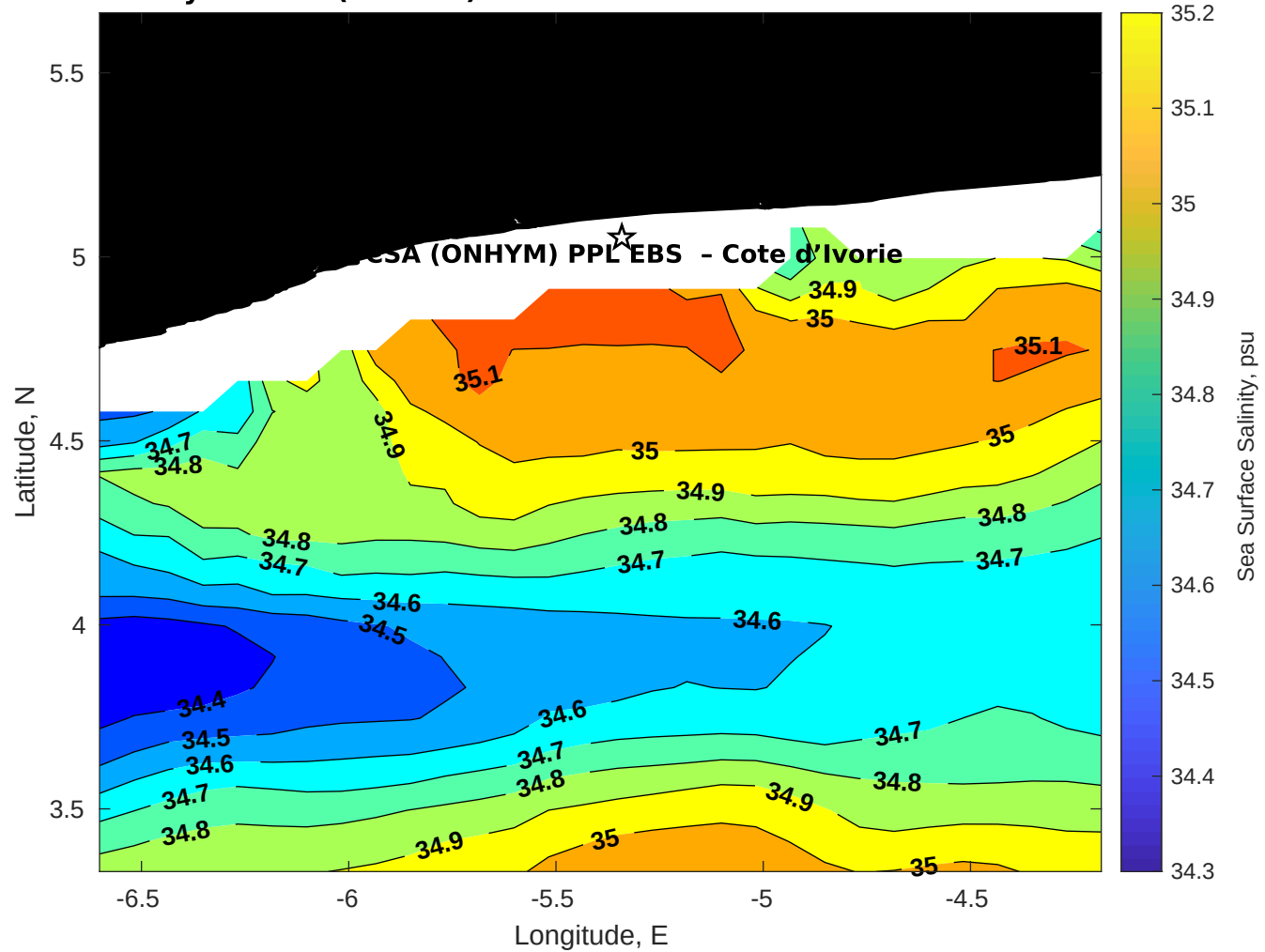
Surface Salinity for CSA (ONHYM) PPL EBS - Cote d'Ivoire at 11-Oct-2025 00:00:00
