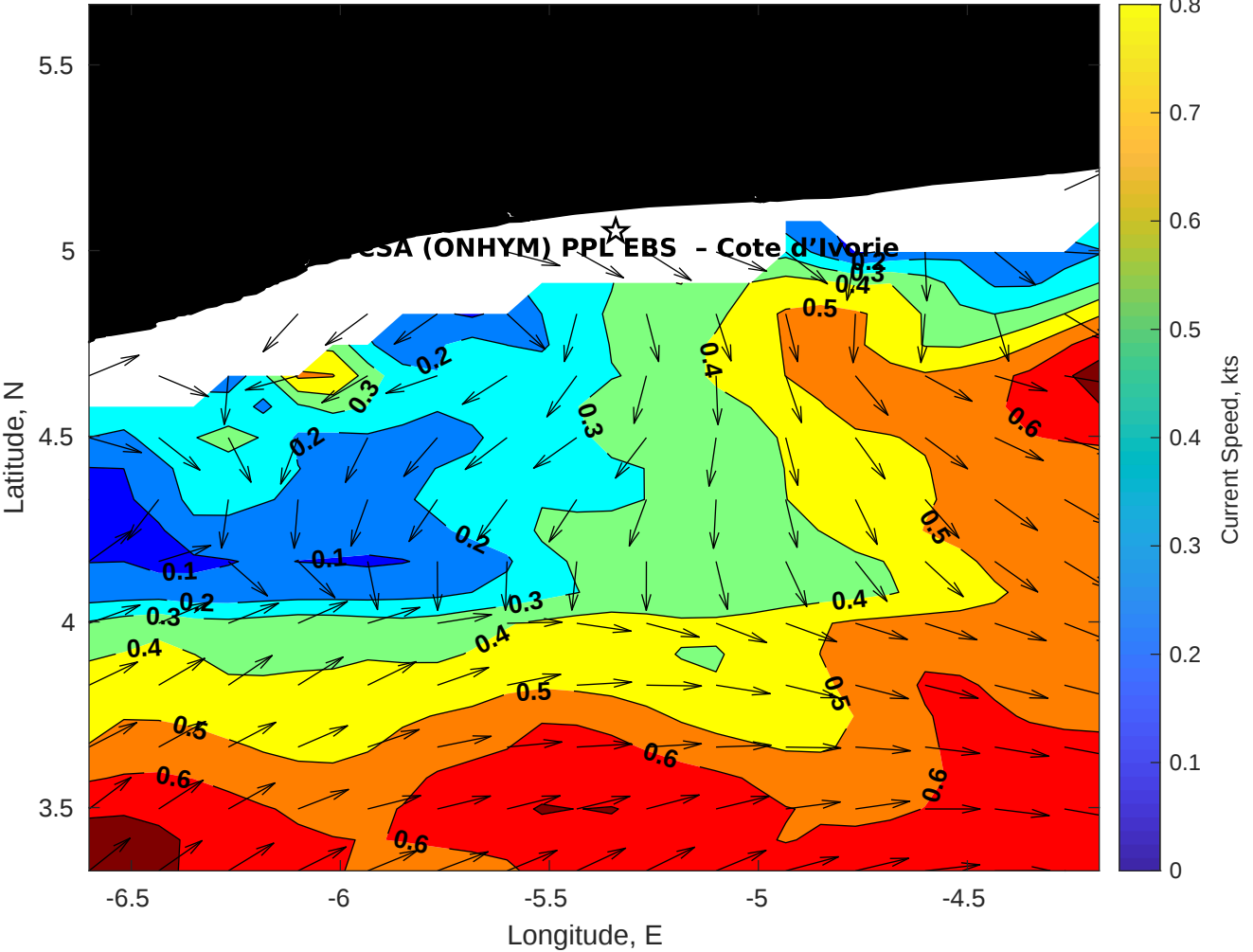
Surface Currents for CSA (ONHYM) PPL EBS - Cote d'Ivoire at 11-Oct-2025 00:00:00
