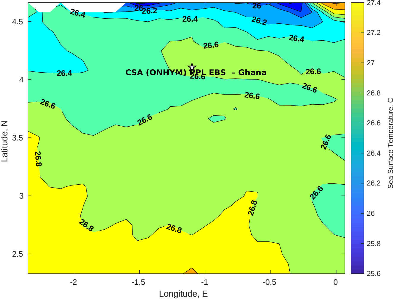
SST for CSA (ONHYM) PPL EBS - Ghana at 11-Oct-2025 00:00:00
