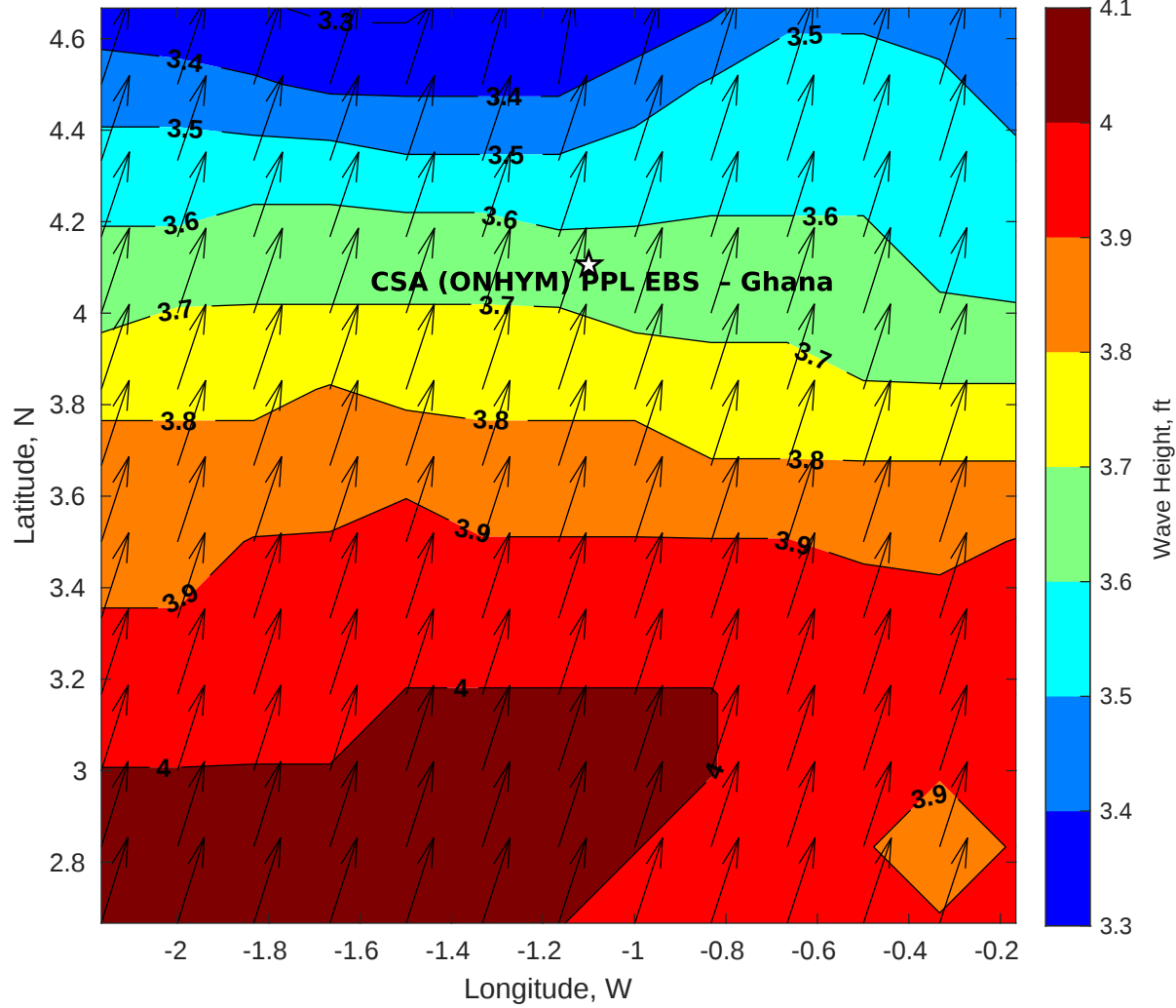
Wave Height (ft) for CSA (ONHYM) PPL EBS - Ghana at 12-Oct-2025 09:00:00
