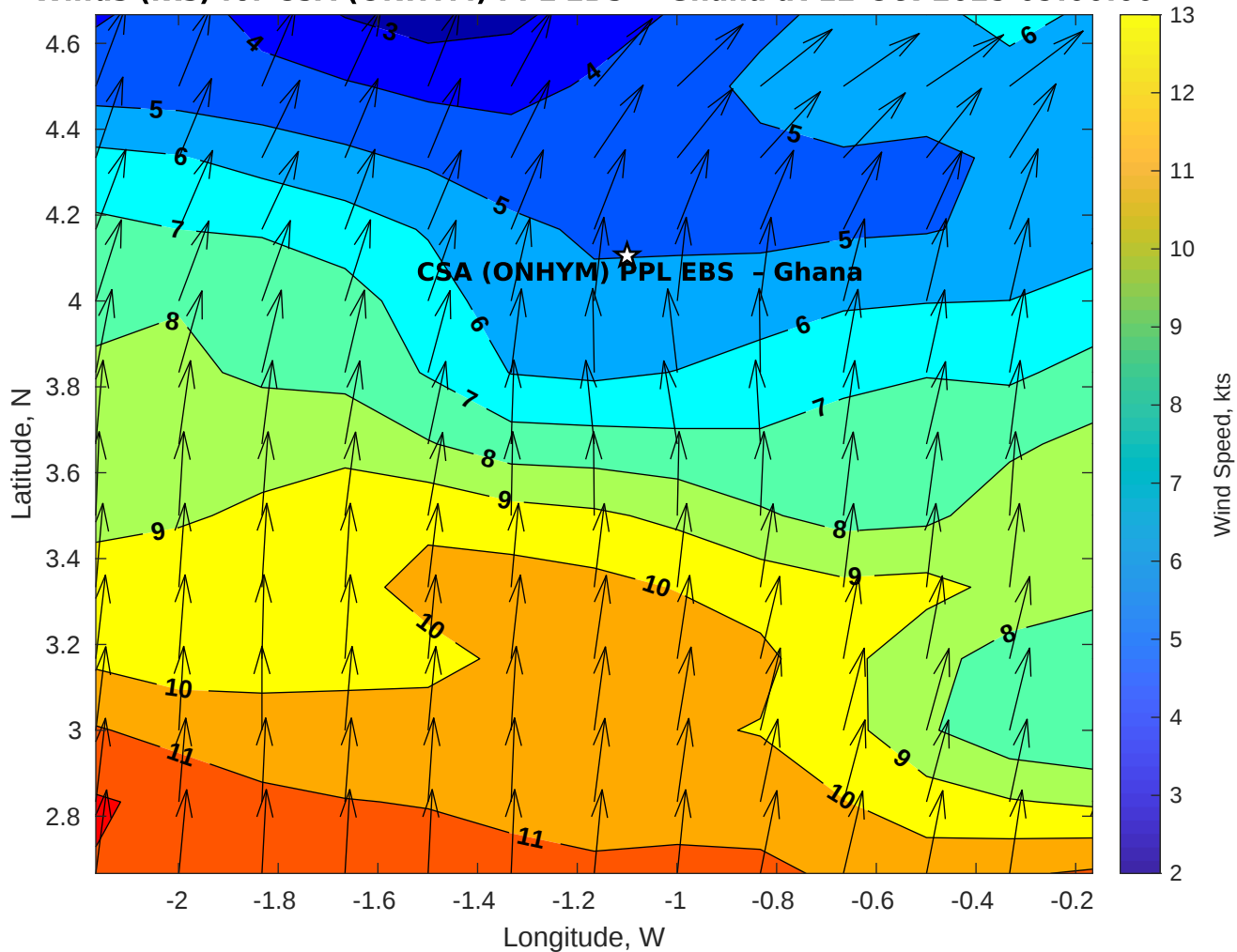
Winds (kts) for CSA (ONHYM) PPL EBS - Ghana at 12-Oct-2025 09:00:00
