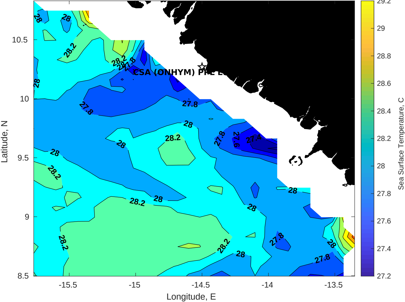
SST for CSA (ONHYM) PPL EBS - Guinea at 11-Oct-2025 00:00:00
