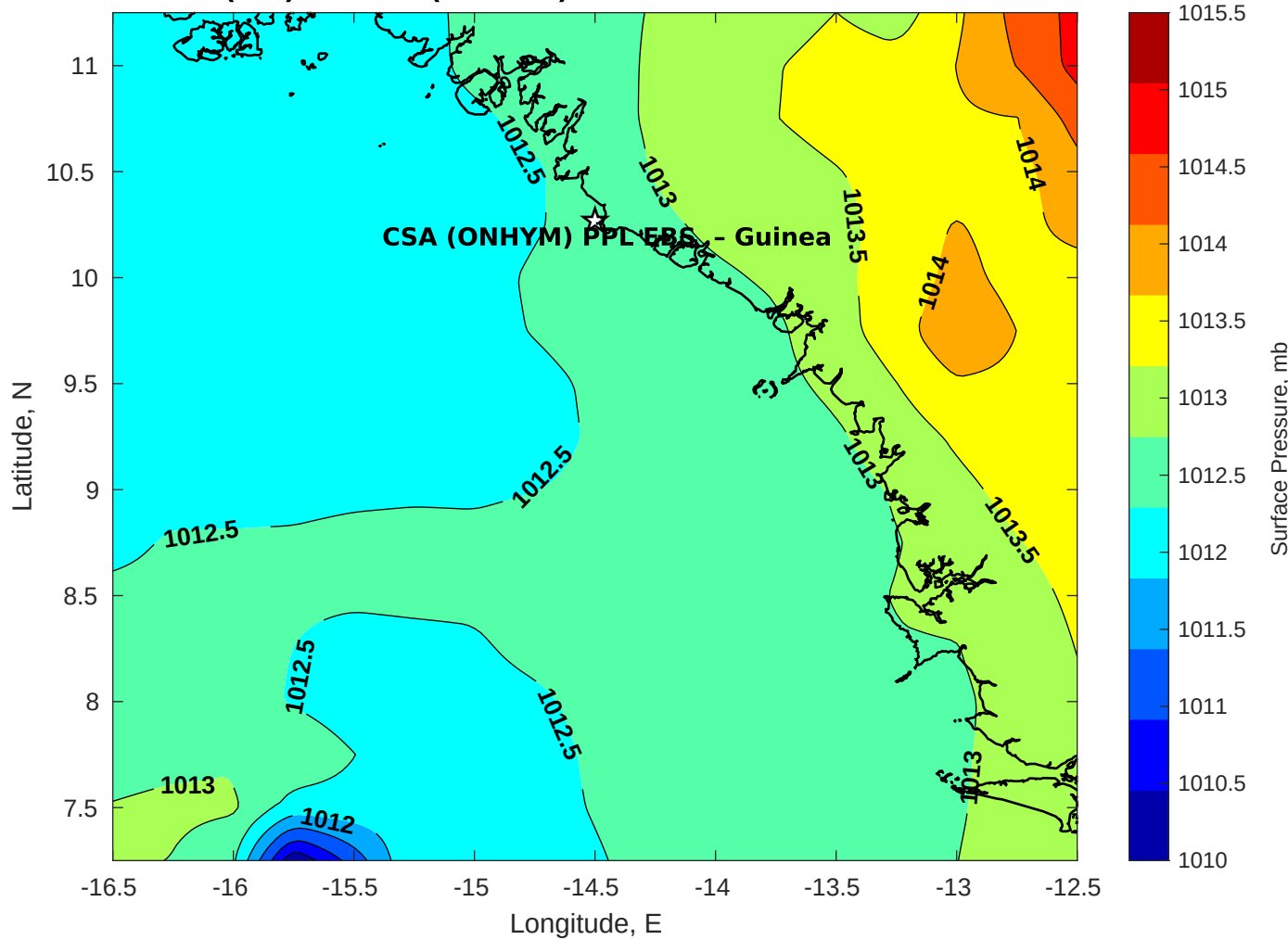
Surface Pressure (mb) for CSA (ONHYM) PPL EBS - Guinea at 14-Oct-2025 00:00:00
