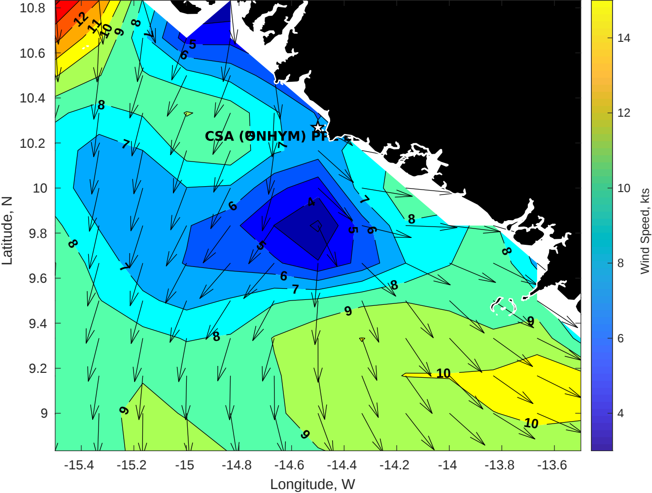
Winds (kts) for CSA (ONHYM) PPL EBS - Guinea at 12-Oct-2025 09:00:00
