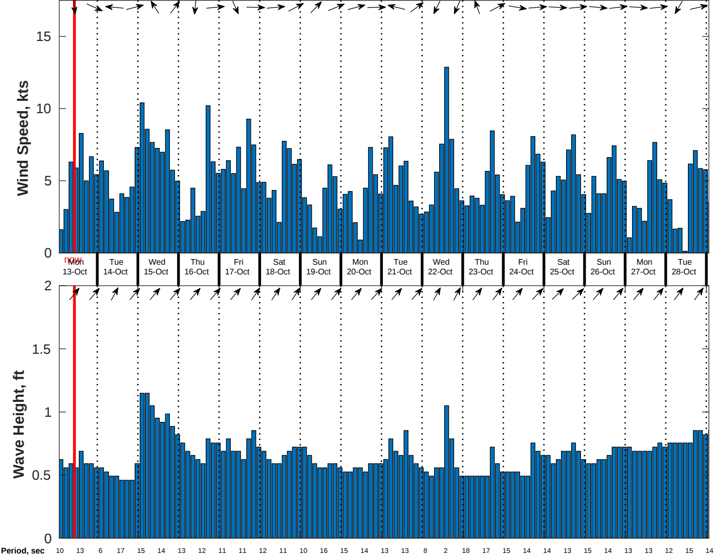
Wind & Wave Forecast for CSA (ONHYM) PPL EBS - Guinea from 12-Oct-2025 01:00:00 to 28-Oct-2025 01:00:00
