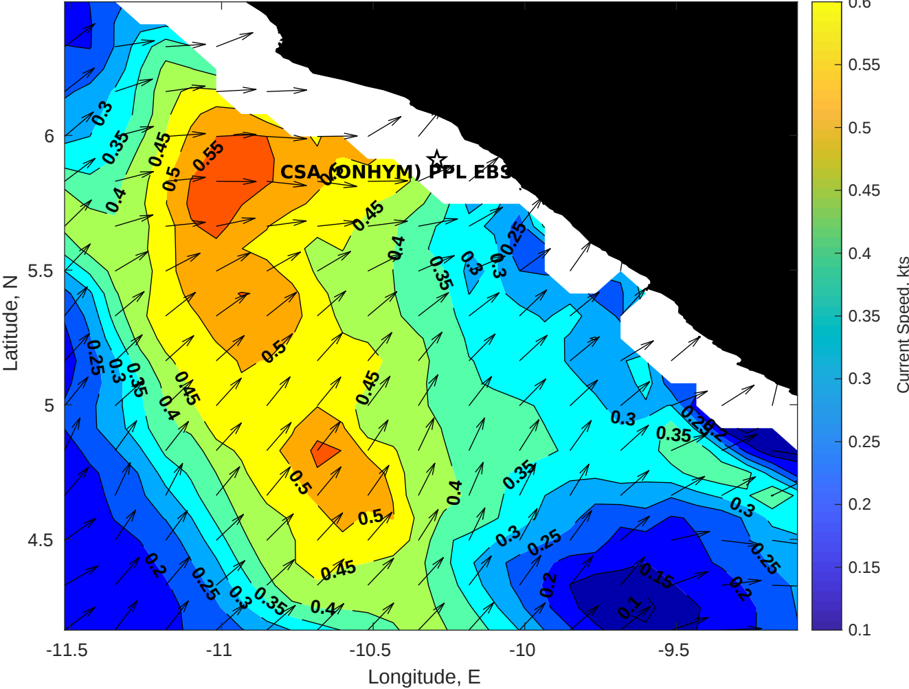
Surface Currents for CSA (ONHYM) PPL EBS - Liberia at 11-Oct-2025 00:00:00
