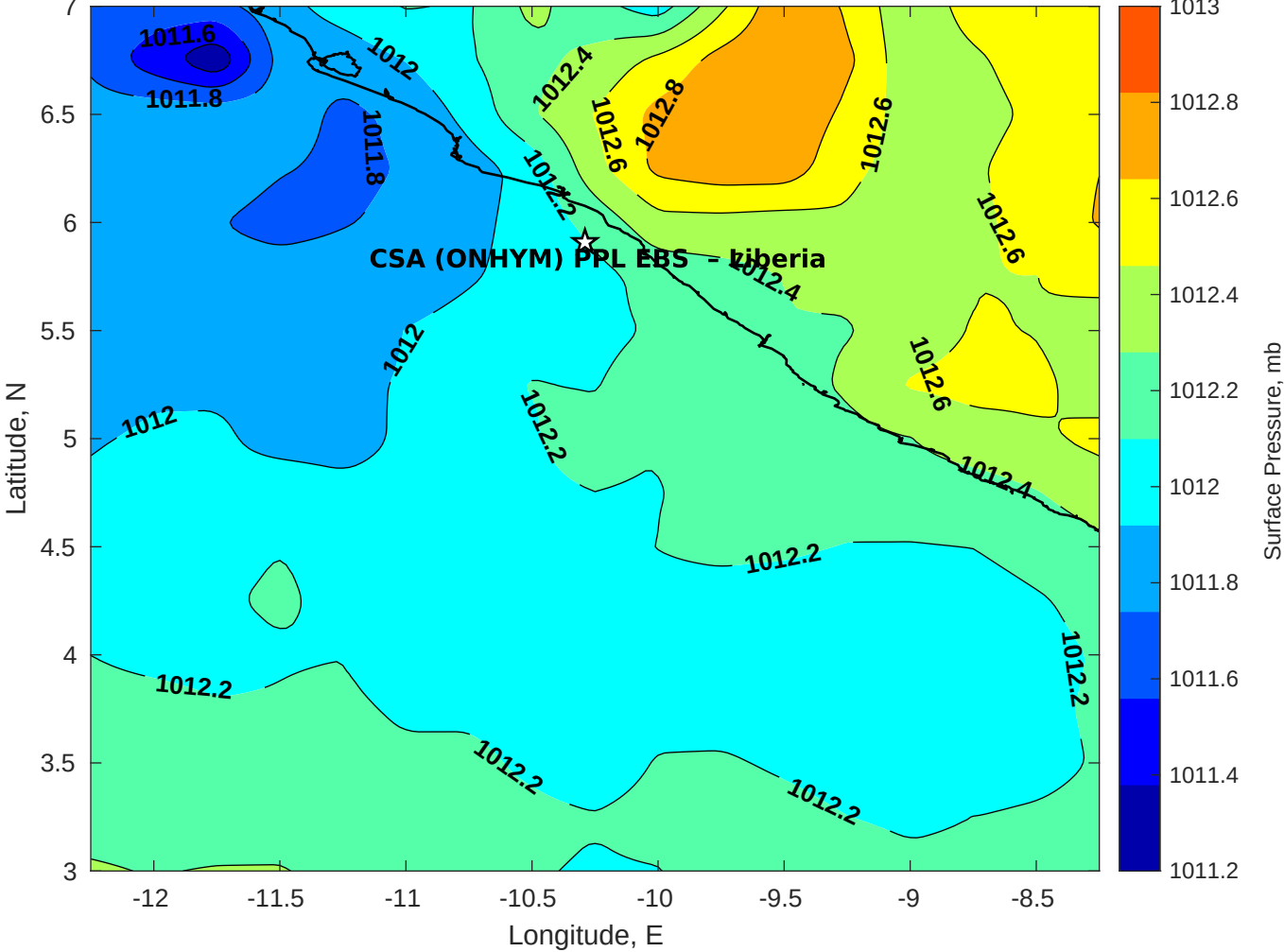
Surface Pressure (mb) for CSA (ONHYM) PPL EBS - Liberia at 13-Oct-2025 00:00:00
