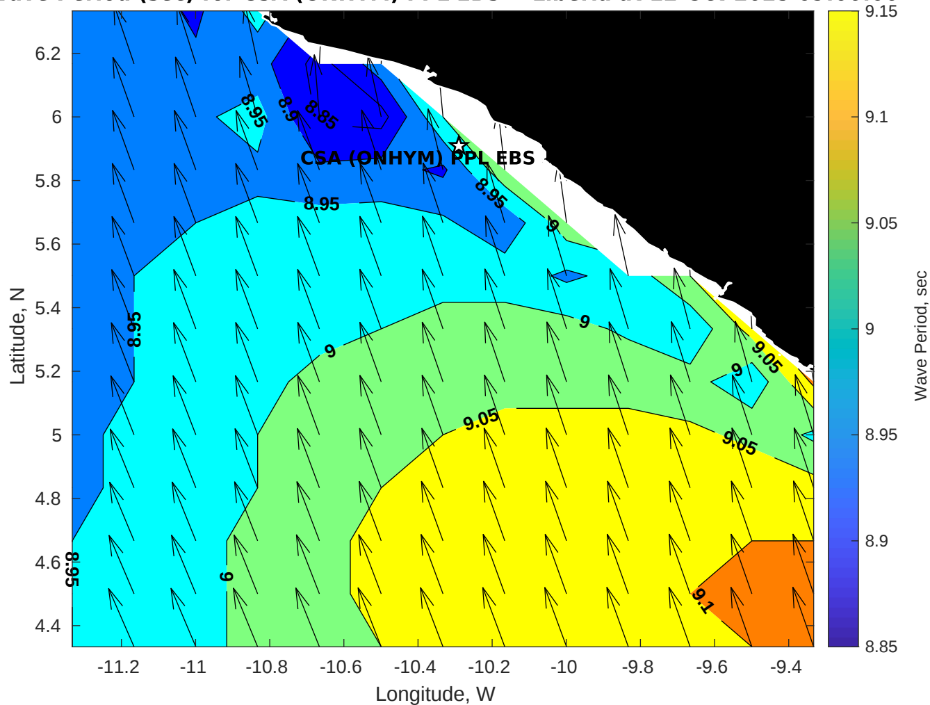
Wave Period (sec) for CSA (ONHYM) PPL EBS - Liberia at 12-Oct-2025 09:00:00
