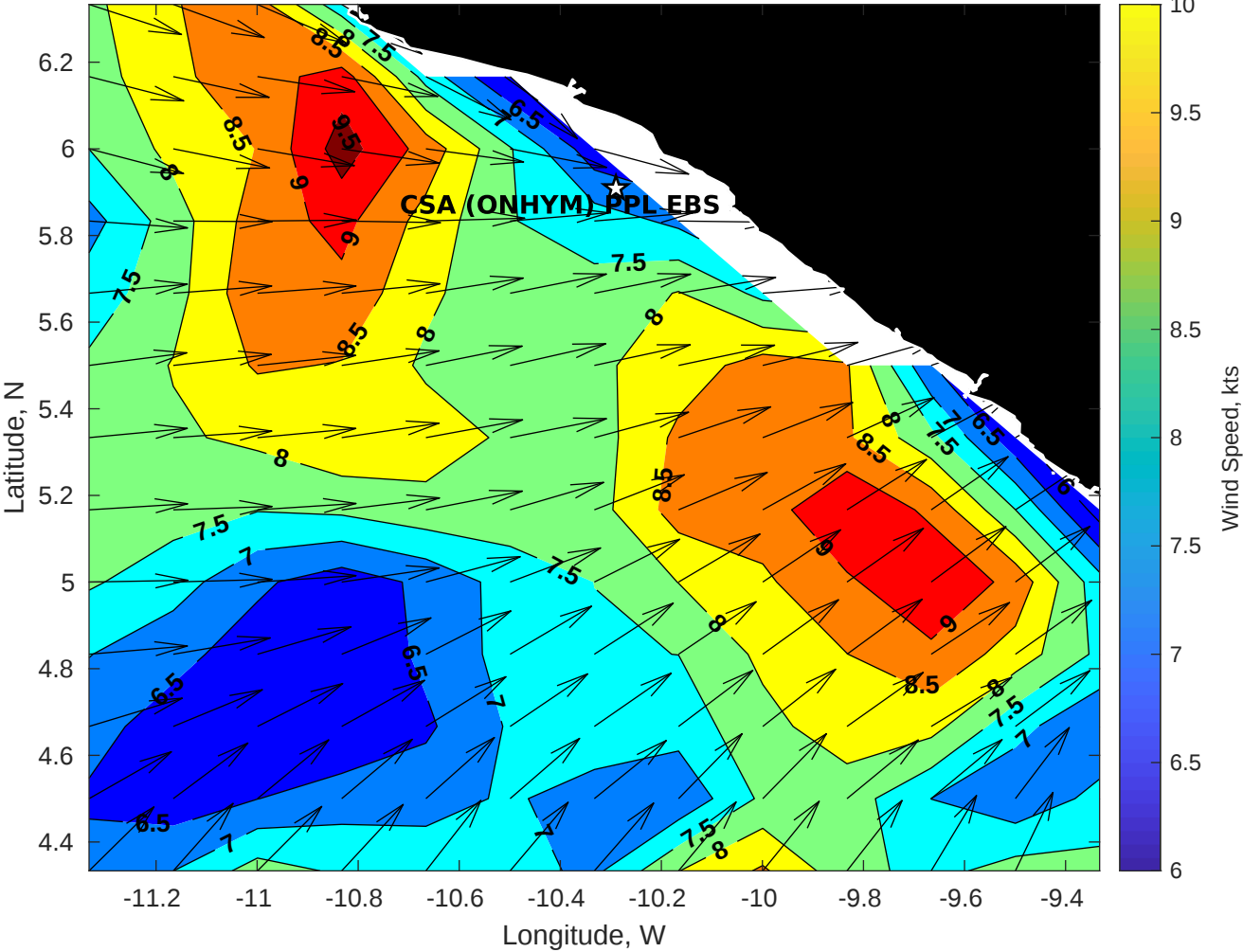
Winds (kts) for CSA (ONHYM) PPL EBS - Liberia at 12-Oct-2025 09:00:00
