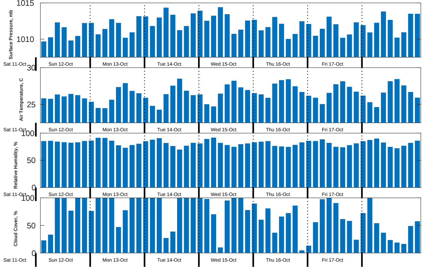
Met Forecast for CSA (ONHYM) PPL EBS - Liberia from 12-Oct-2025 00:00:00 to 19-Oct-2025 00:00:00
