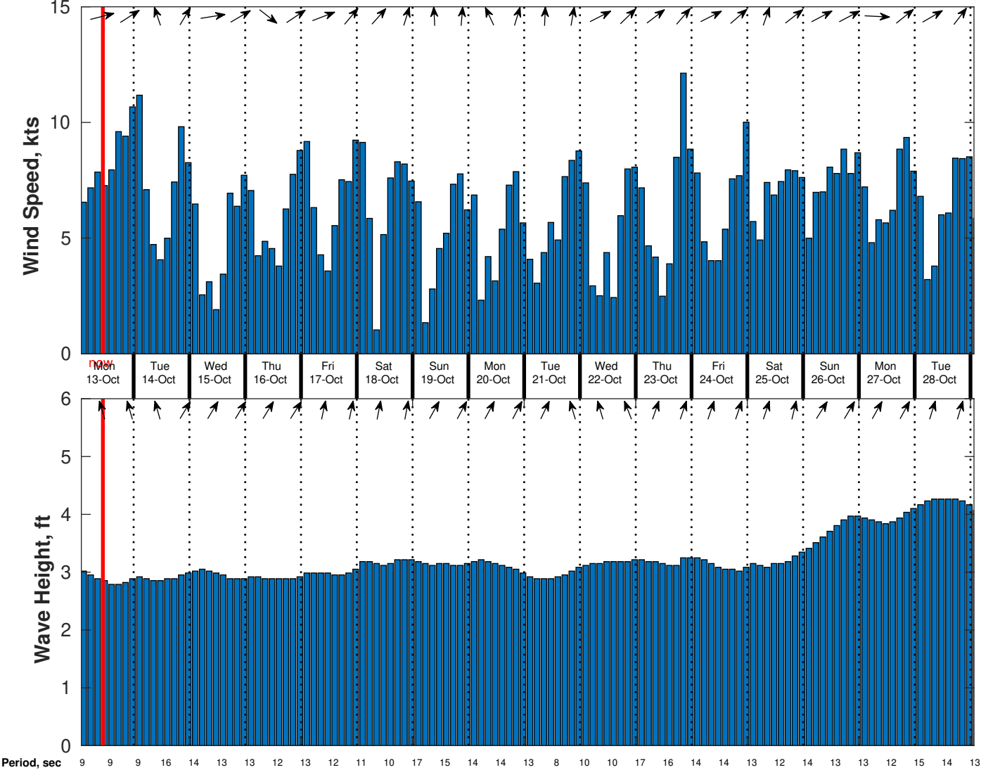
Wind & Wave Forecast for CSA (ONHYM) PPL EBS - Liberia from 12-Oct-2025 01:00:00 to 28-Oct-2025 01:00:00
