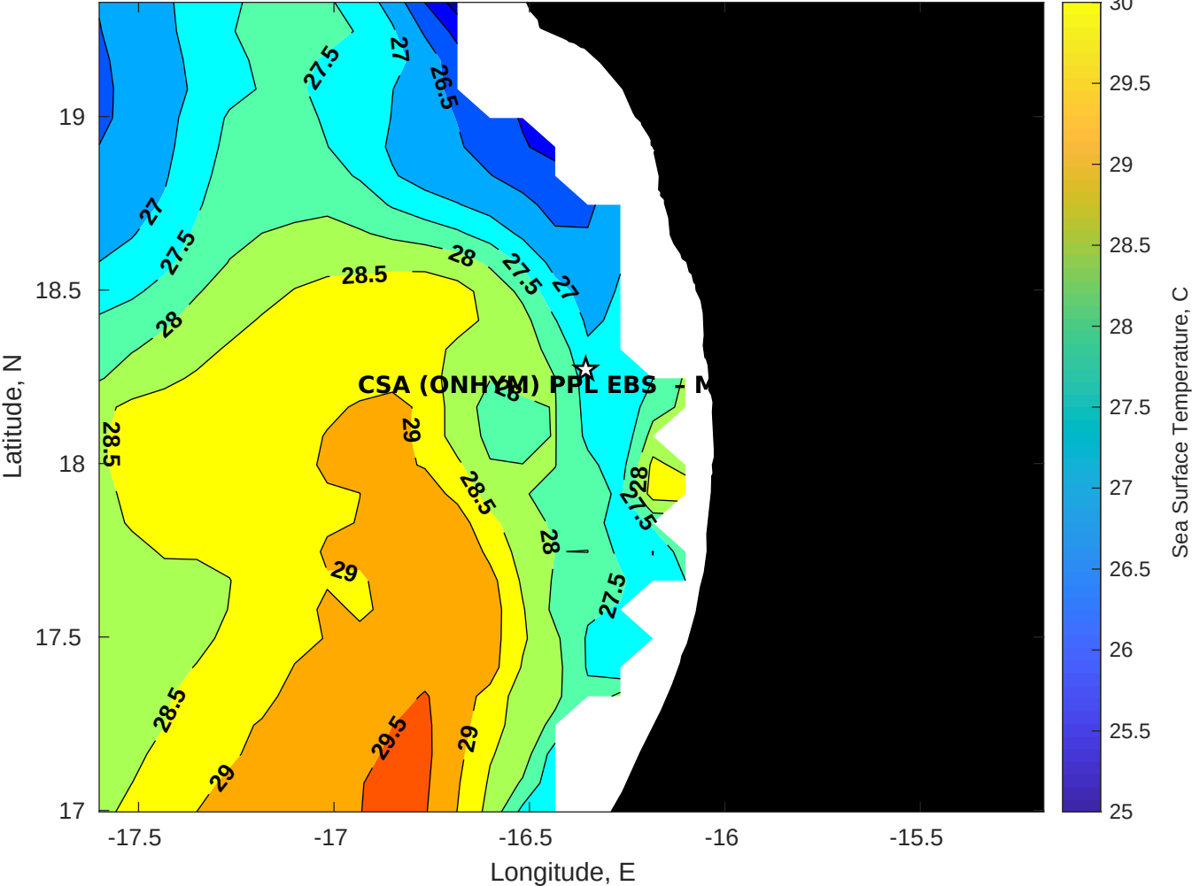
SST for CSA (ONHYM) PPL EBS - Mauritania at 11-Oct-2025 00:00:00
