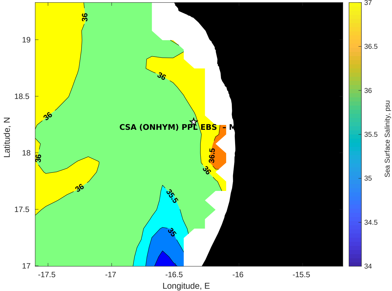
Surface Salinity for CSA (ONHYM) PPL EBS - Mauritania at 11-Oct-2025 00:00:00
