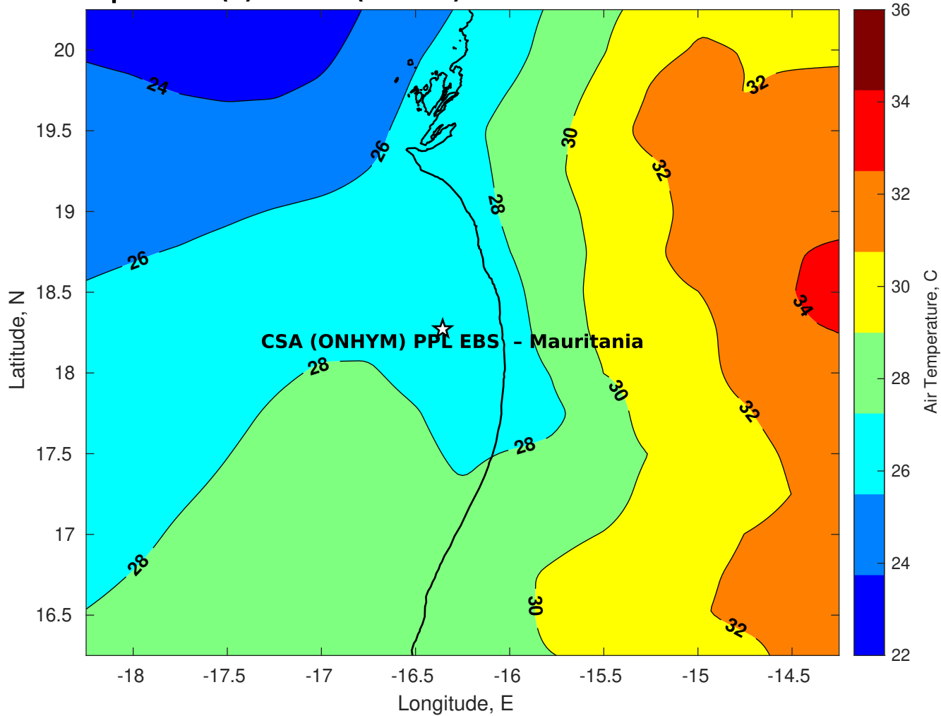
Air Temperature (C) for CSA (ONHYM) PPL EBS - Mauritania at 12-Oct-2025
