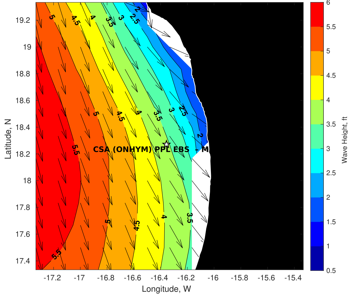
Wave Height (ft) for CSA (ONHYM) PPL EBS - Mauritania at 12-Oct-2025 09:00:00
