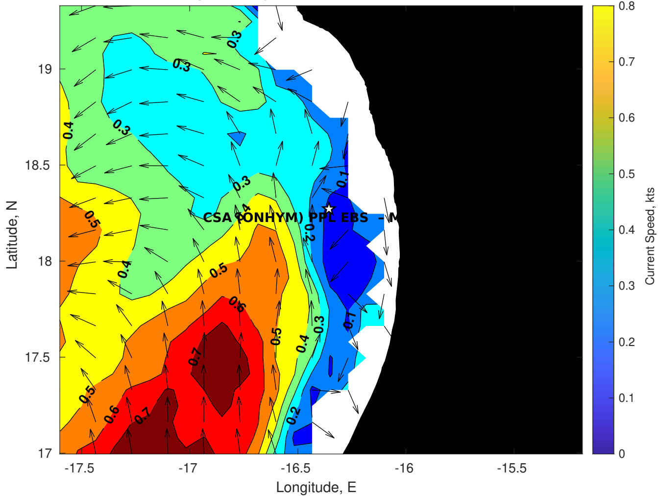
Surface Currents for CSA (ONHYM) PPL EBS - Mauritania at 11-Oct-2025 00:00:00
