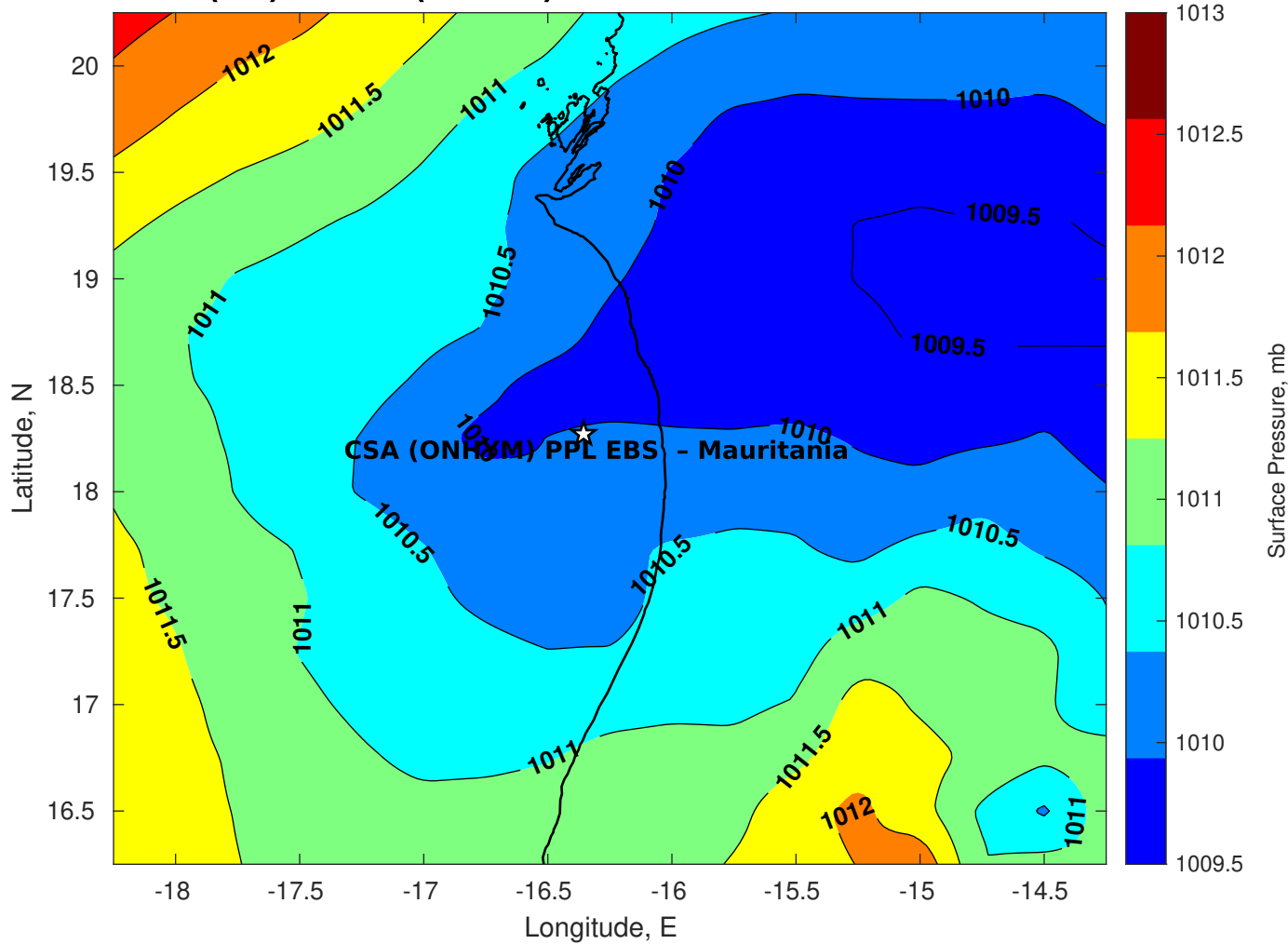
Surface Pressure (mb) for CSA (ONHYM) PPL EBS - Mauritania at 12-Oct-2025 00:00:00
