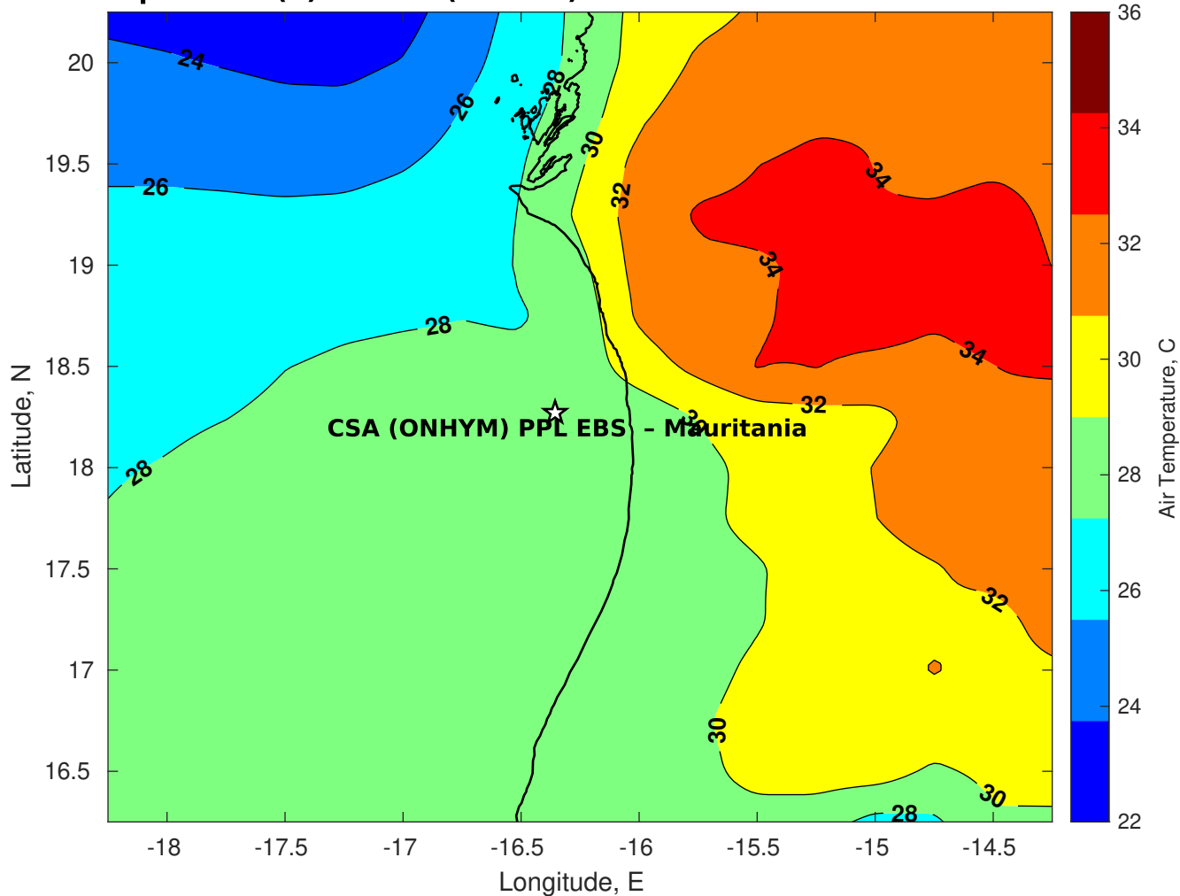
Air Temperature (C) for CSA (ONHYM) PPL EBS - Mauritania at 12-Oct-2025
