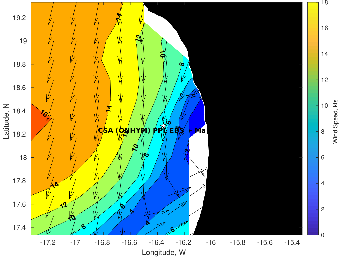
Winds (kts) for CSA (ONHYM) PPL EBS - Mauritania at 12-Oct-2025 09:00:00
