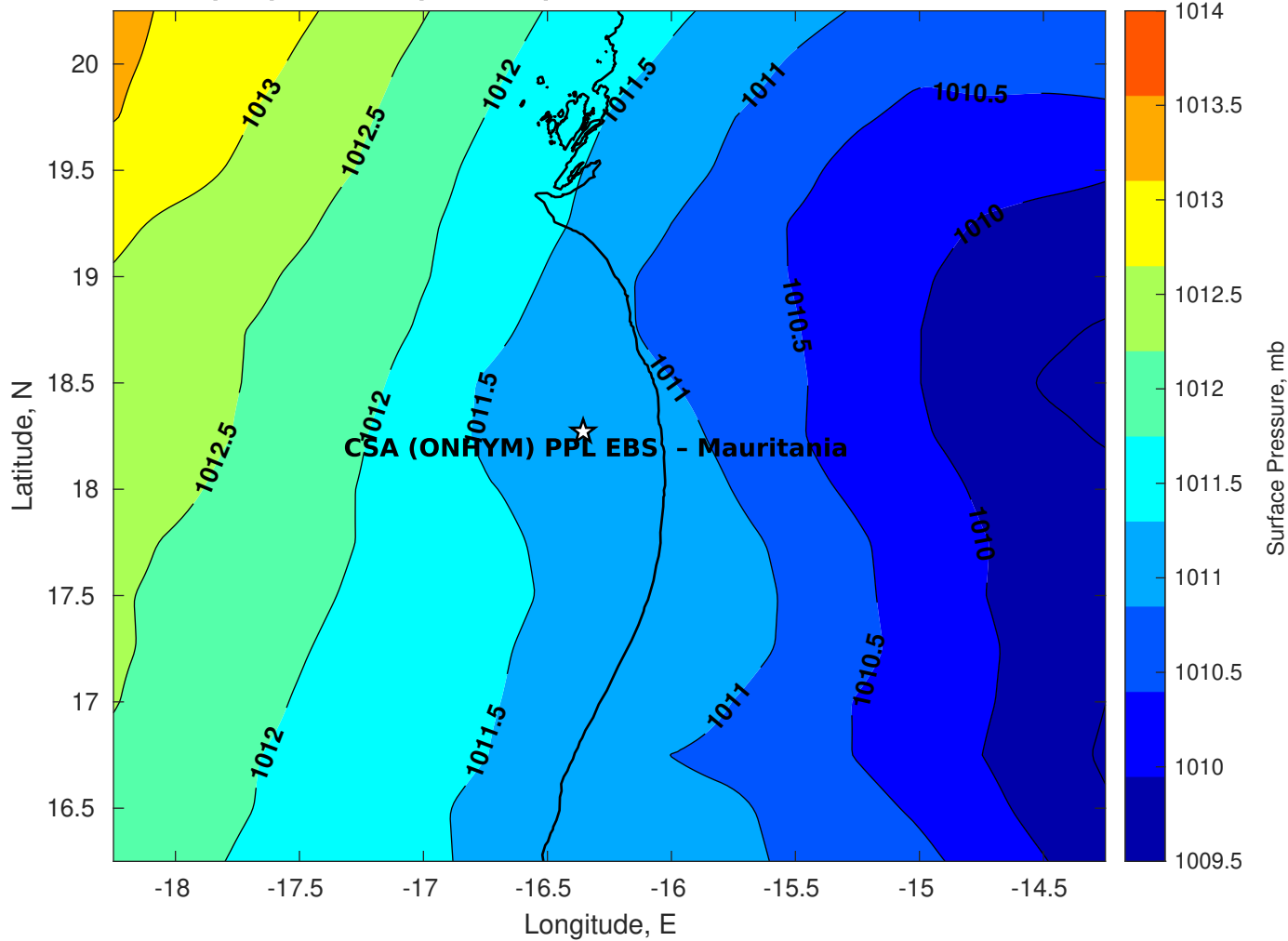
Surface Pressure (mb) for CSA (ONHYM) PPL EBS - Mauritania at 13-Oct-2025 00:00:00
