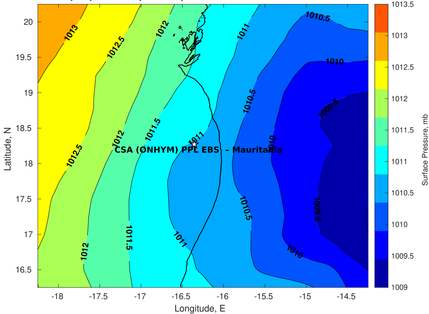
Surface Pressure (mb) for CSA (ONHYM) PPL EBS - Mauritania at 14-Oct-2025 00:00:00
