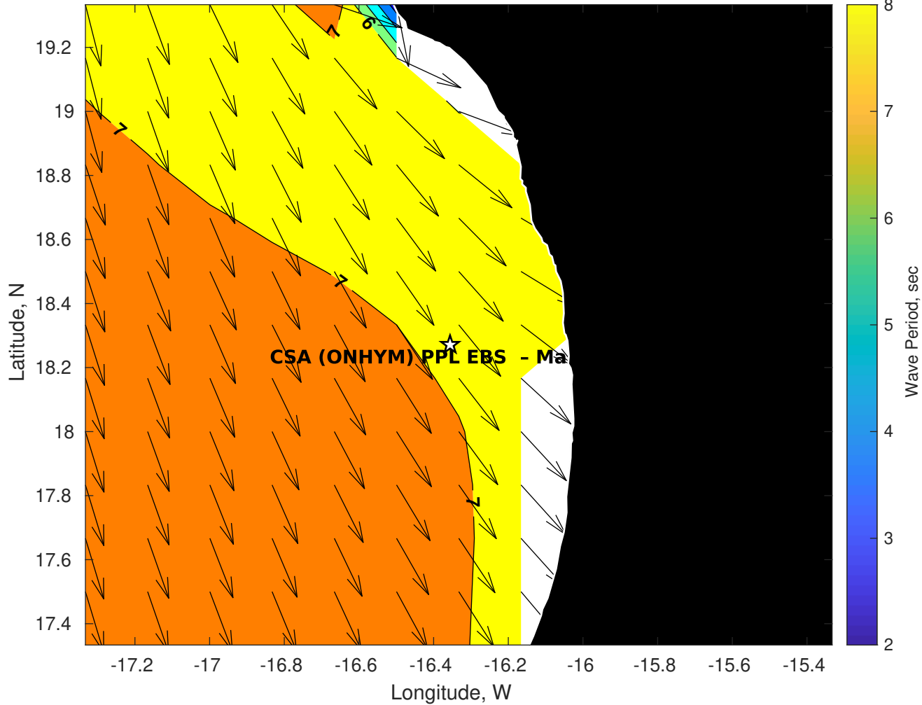
Wave Period (sec) for CSA (ONHYM) PPL EBS - Mauritania at 12-Oct-2025 09:00:00
