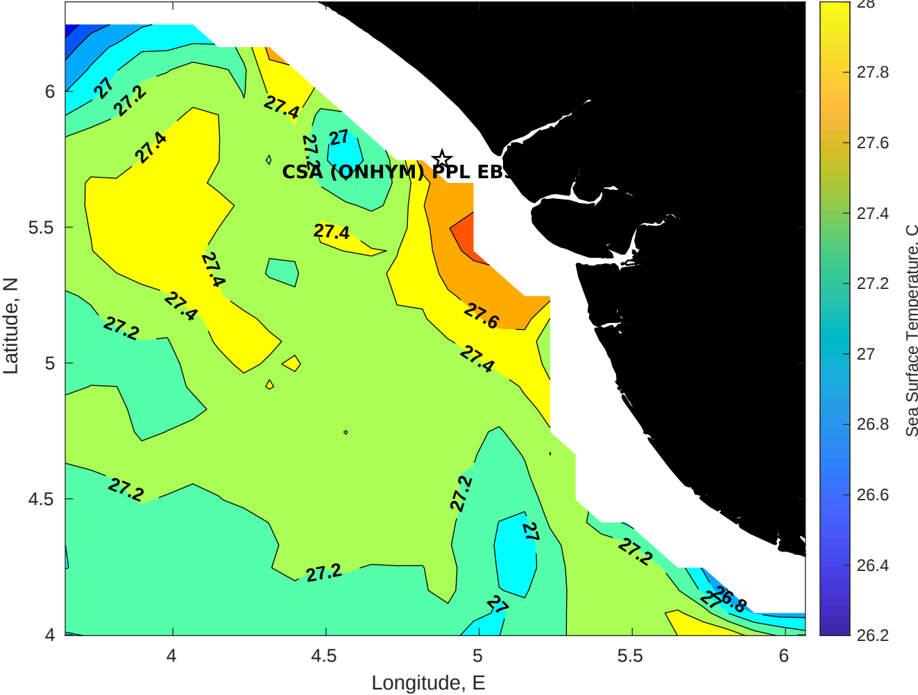
SST for CSA (ONHYM) PPL EBS - Nigeria at 11-Oct-2025 00:00:00
