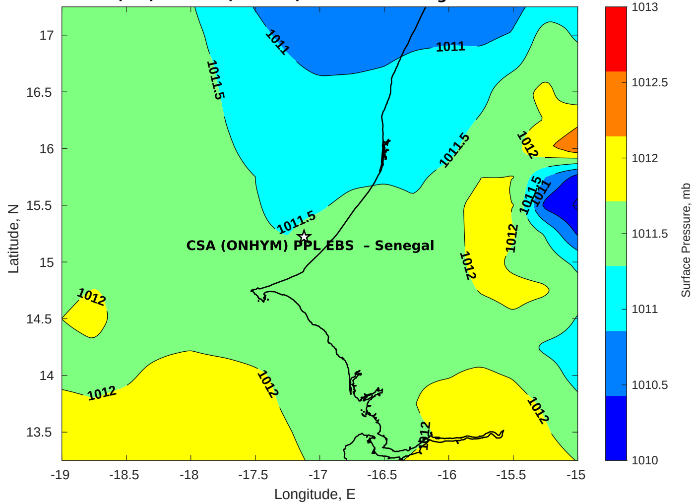
Surface Pressure (mb) for CSA (ONHYM) PPL EBS - Senegal at 12-Oct-2025 00:00:00
