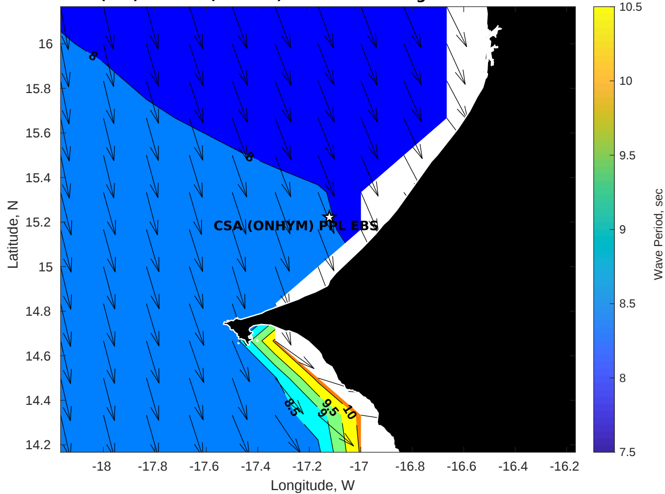
Wave Period (sec) for CSA (ONHYM) PPL EBS - Senegal at 12-Oct-2025 09:00:00
