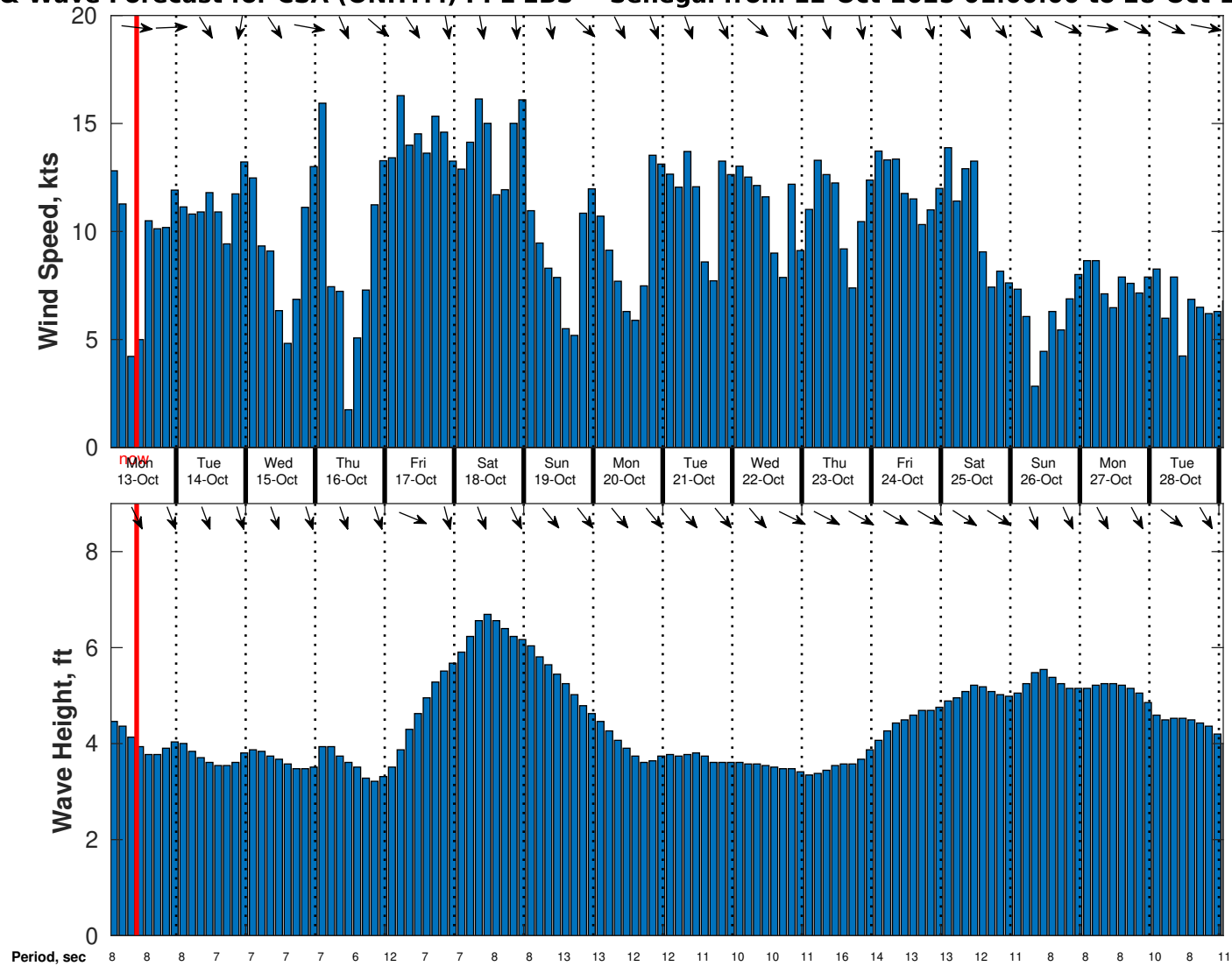
Wind & Wave Forecast for CSA (ONHYM) PPL EBS - Senegal from 12-Oct-2025 01:00:00 to 28-Oct-2025 01:00:00
