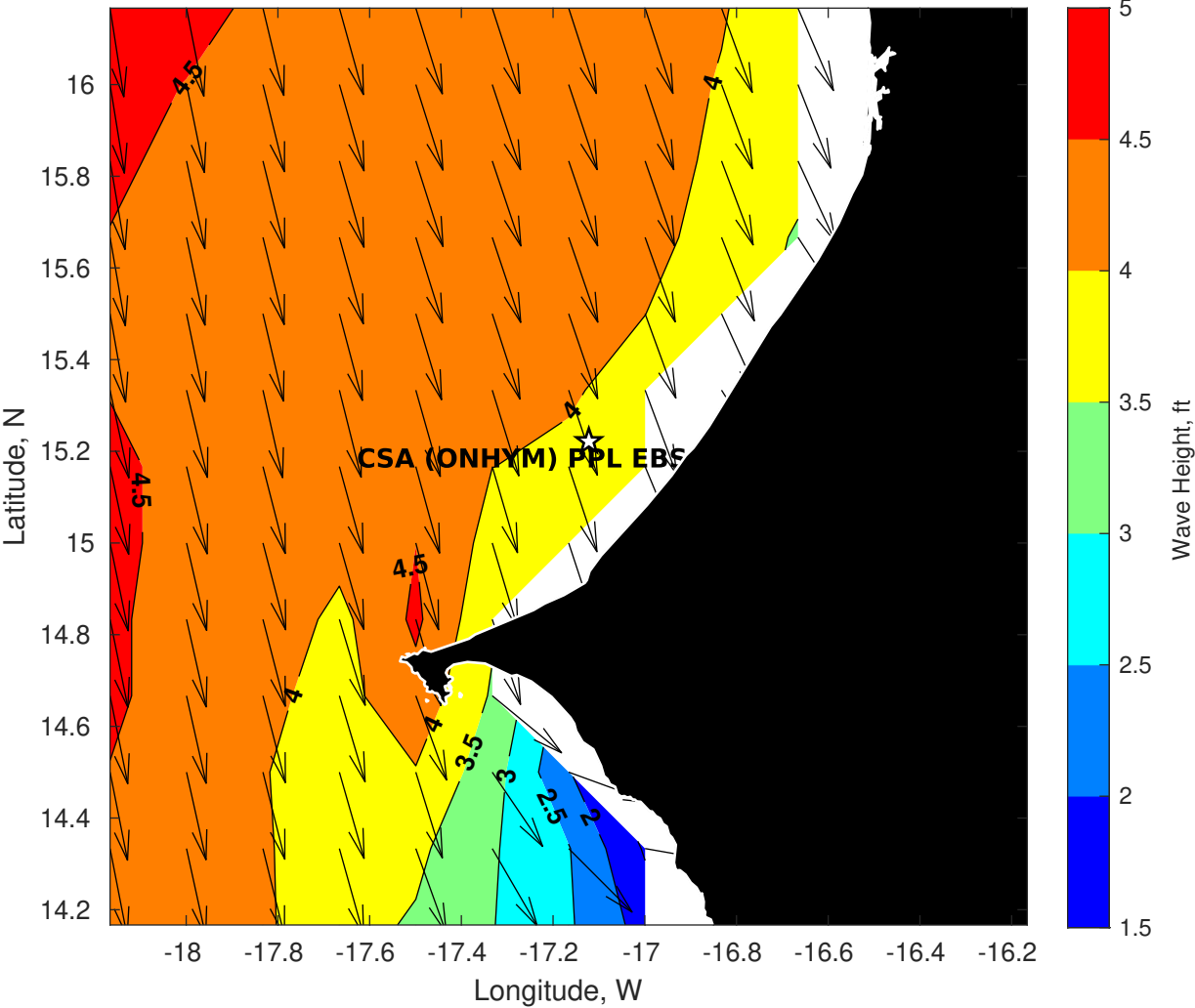
Wave Height (ft) for CSA (ONHYM) PPL EBS - Senegal at 12-Oct-2025 09:00:00
