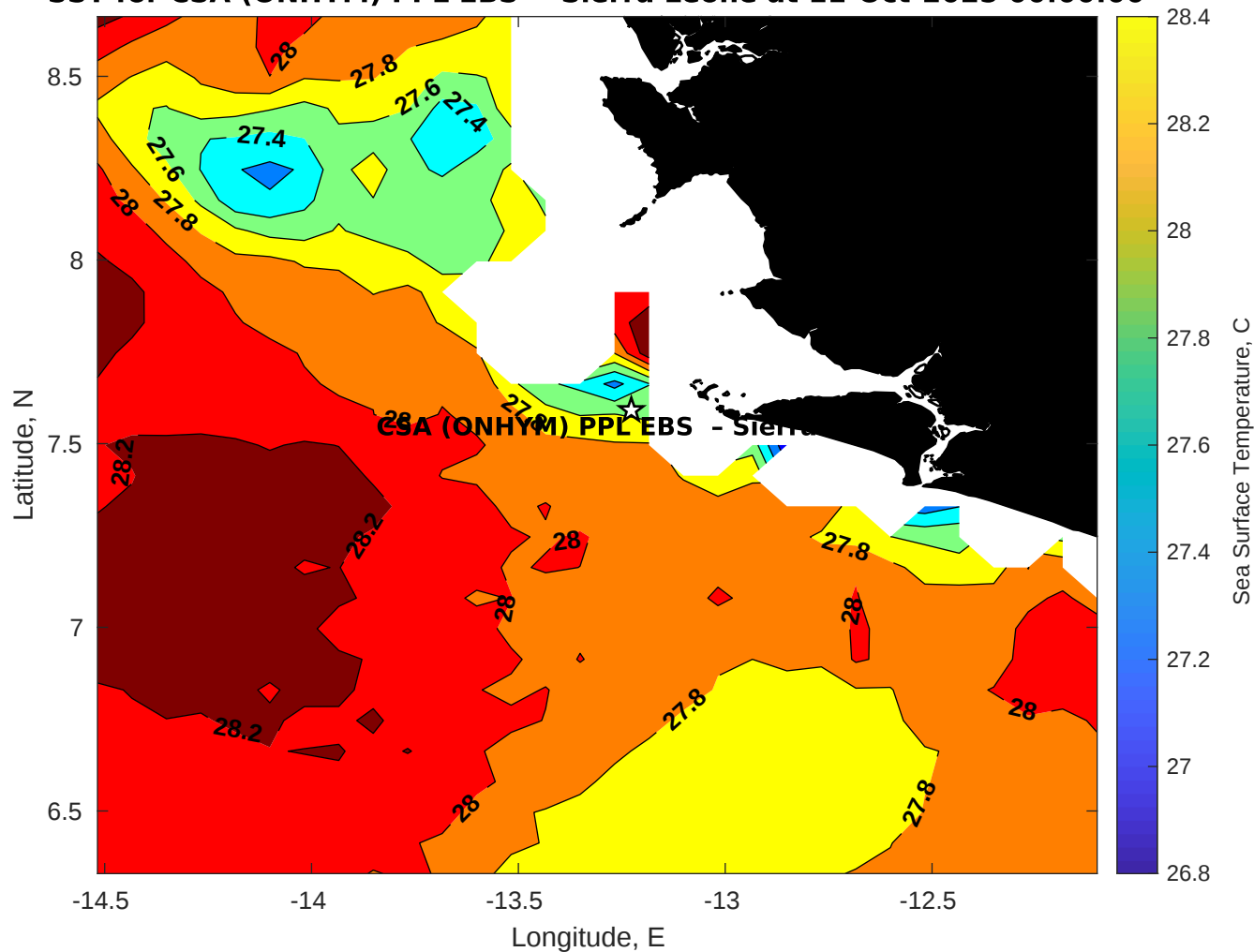
SST for CSA (ONHYM) PPL EBS - Sierra Leone at 11-Oct-2025 00:00:00
