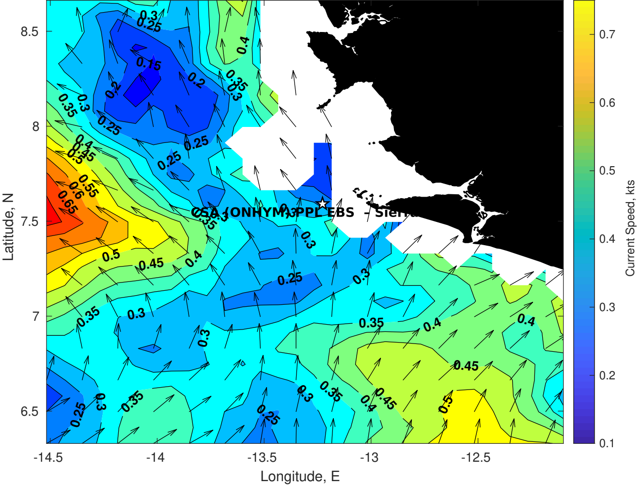
Surface Currents for CSA (ONHYM) PPL EBS - Sierra Leone at 11-Oct-2025 00:00:00
