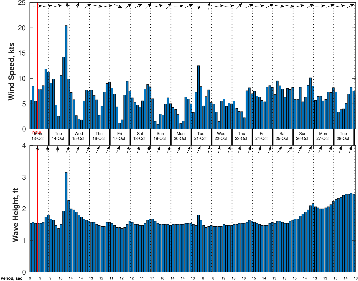
Wind & Wave Forecast for CSA (ONHYM) PPL EBS - Sierra Leone from 12-Oct-2025 01:00:00 to 28-Oct-2025 01:00:00
