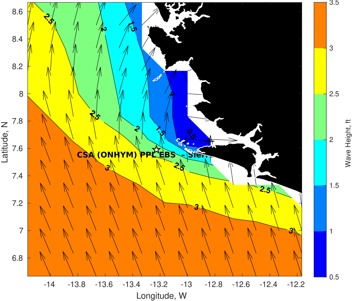
Wave Height (ft) for CSA (ONHYM) PPL EBS - Sierra Leone at 12-Oct-2025 09:00:00
