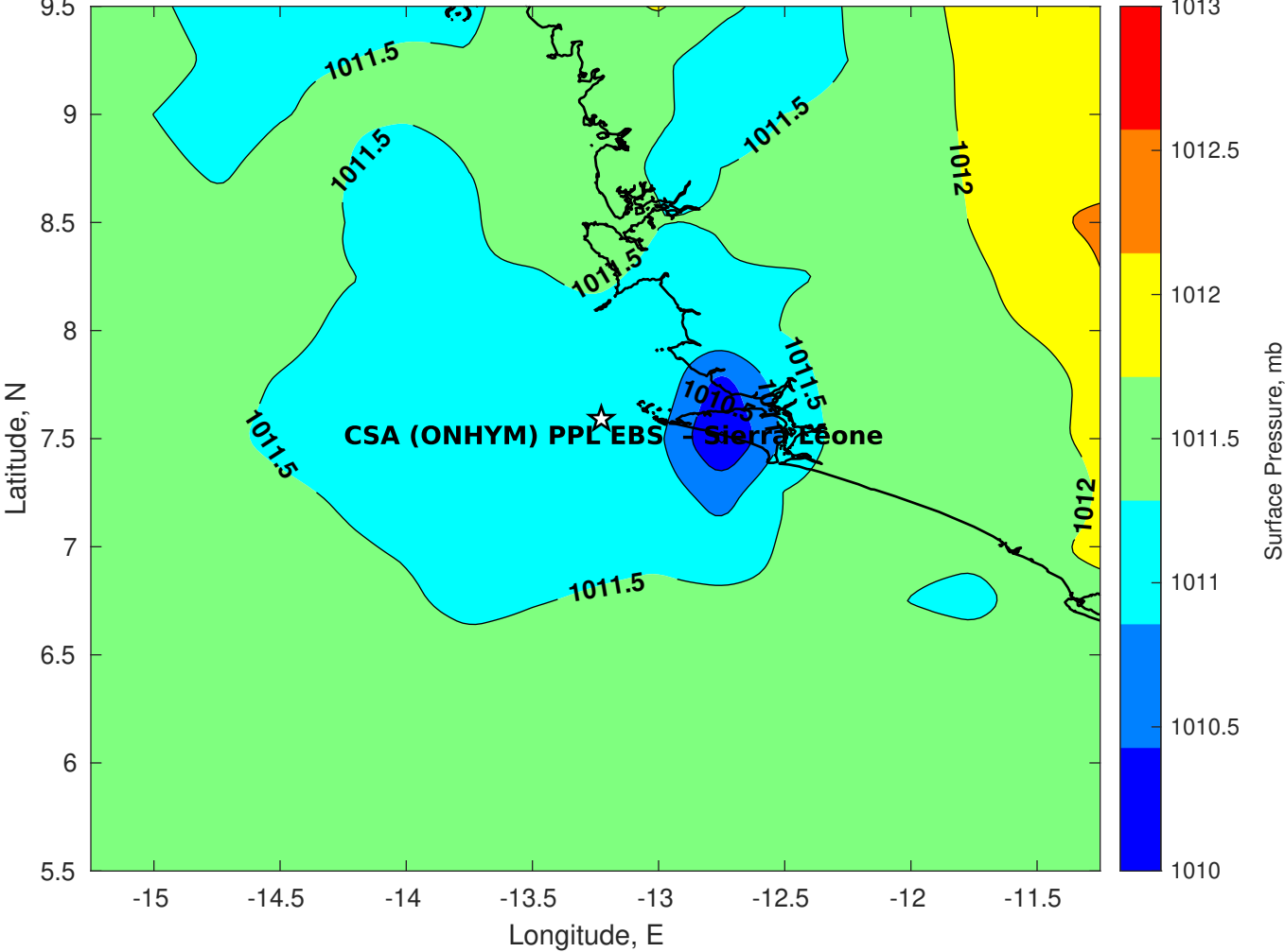
Surface Pressure (mb) for CSA (ONHYM) PPL EBS - Sierra Leone at 13-Oct-2025 00:00:00
