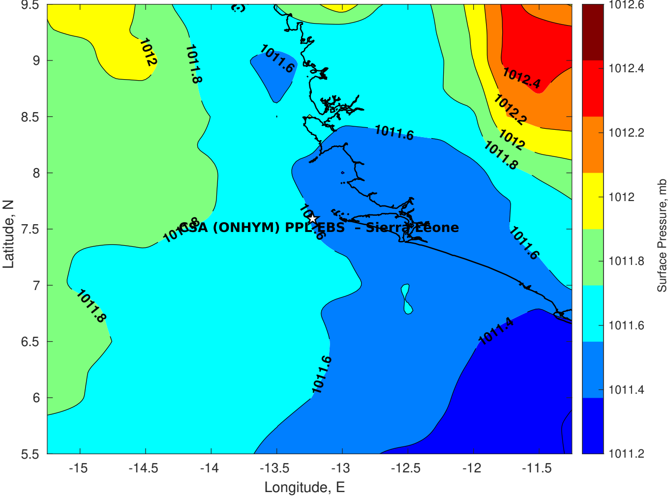
Surface Pressure (mb) for CSA (ONHYM) PPL EBS - Sierra Leone at 12-Oct-2025 00:00:00
