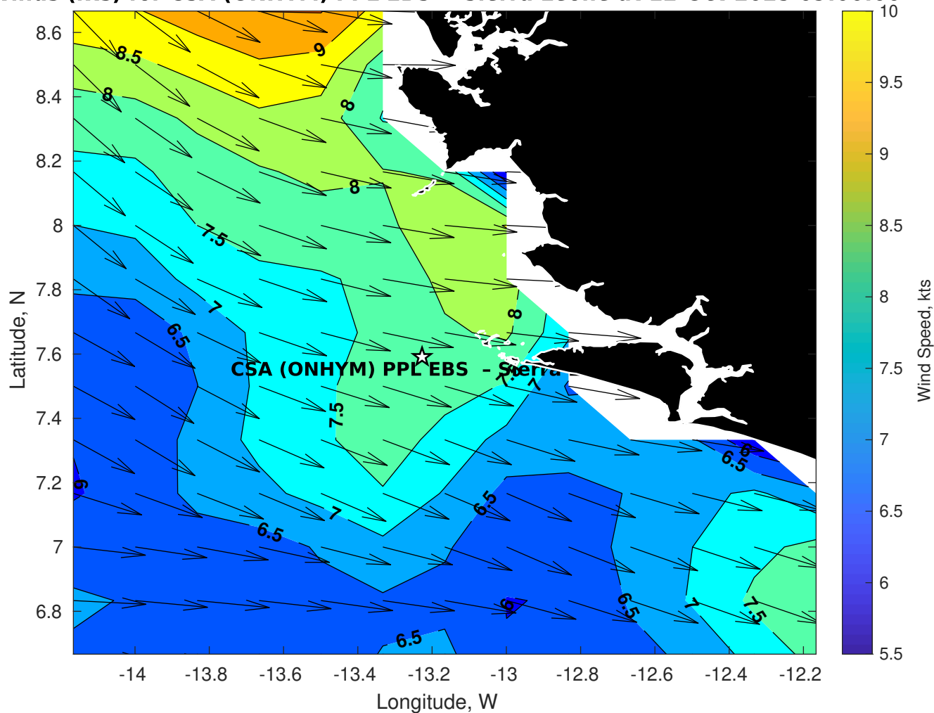
Winds (kts) for CSA (ONHYM) PPL EBS - Sierra Leone at 12-Oct-2025 09:00:00
