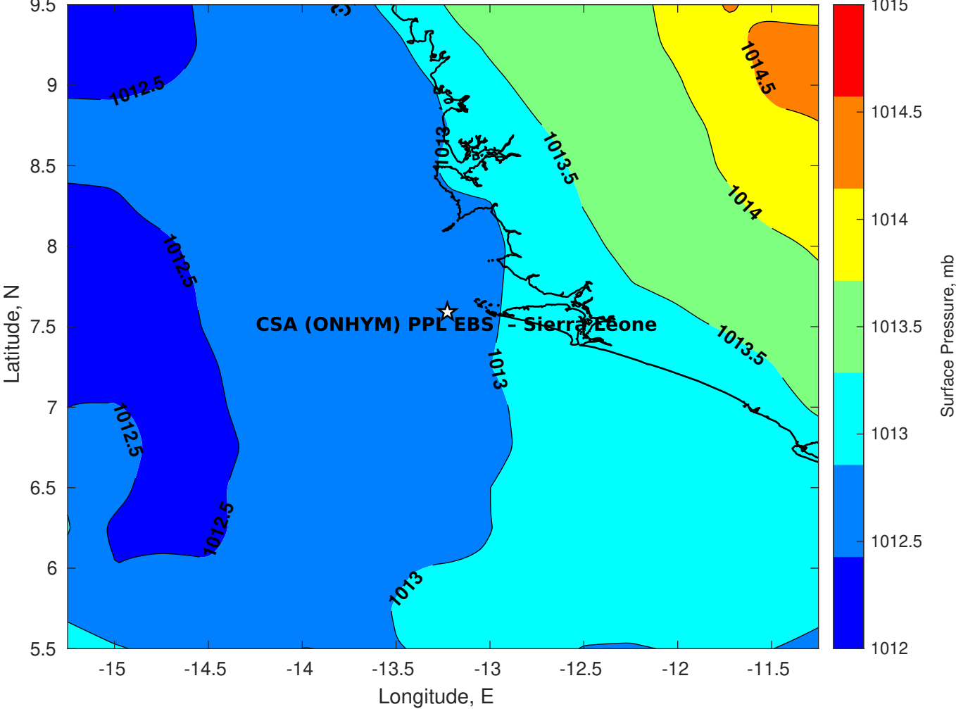
Surface Pressure (mb) for CSA (ONHYM) PPL EBS - Sierra Leone at 14-Oct-2025 00:00:00
