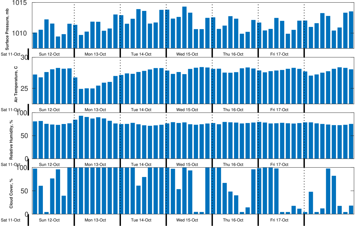
Met Forecast for CSA (ONHYM) PPL EBS - Sierra Leone from 12-Oct-2025 00:00:00 to 19-Oct-2025 00:00:00
