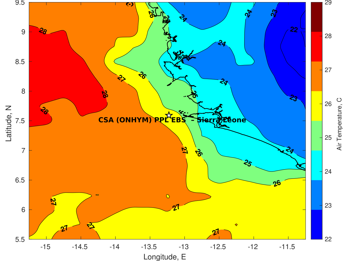
Air Temperature (C) for CSA (ONHYM) PPL EBS - Sierra Leone at 12-Oct-2025
