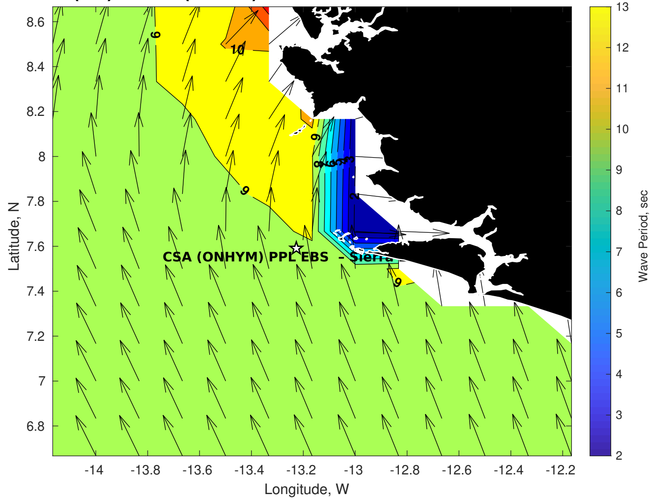
Wave Period (sec) for CSA (ONHYM) PPL EBS - Sierra Leone at 12-Oct-2025 09:00:00
