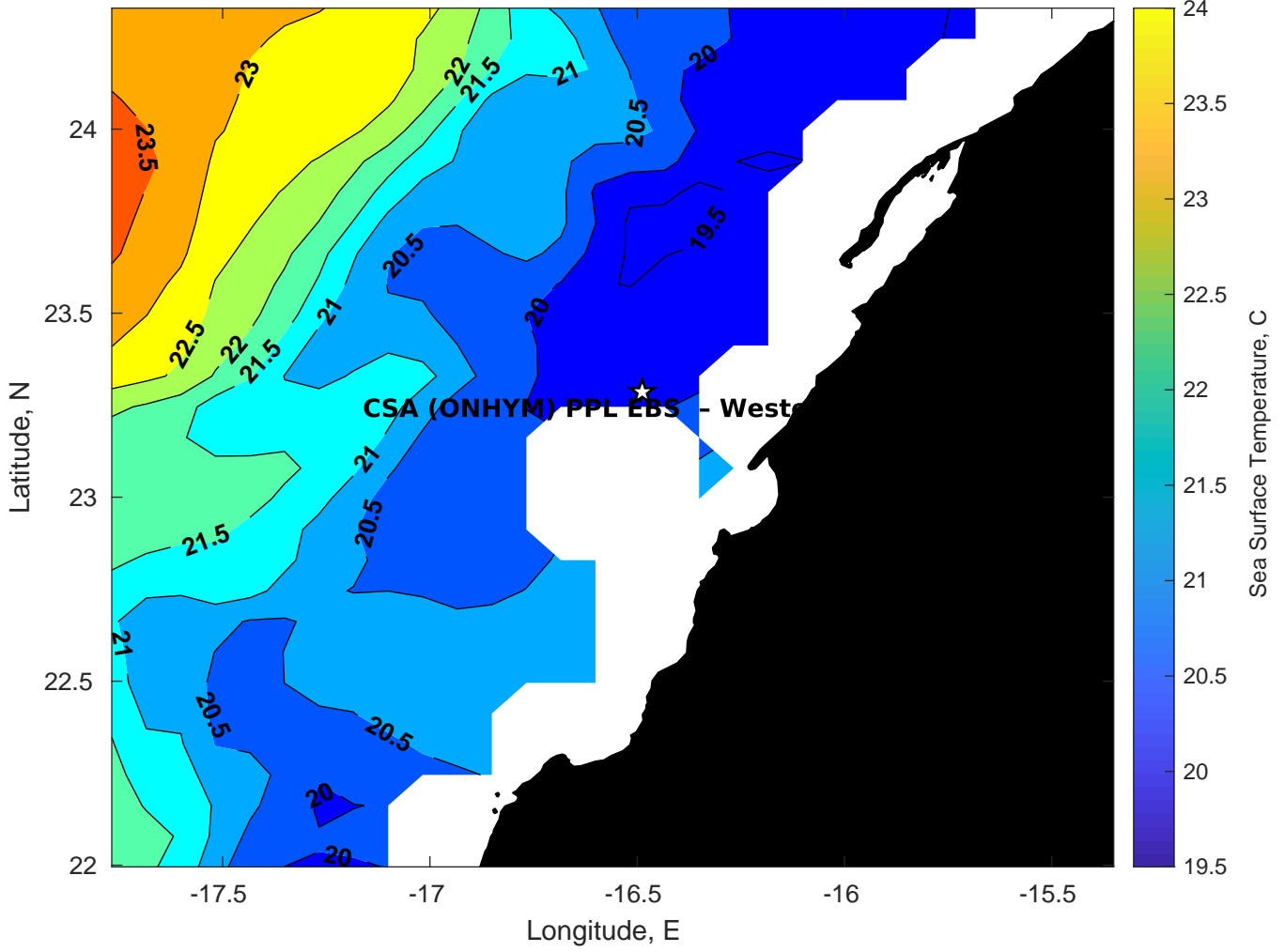
SST for CSA (ONHYM) PPL EBS - Western Sahara at 11-Oct-2025 00:00:00
