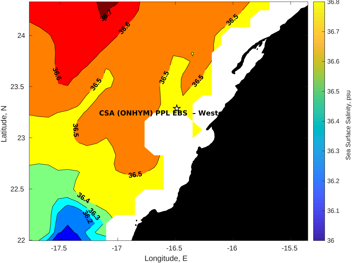
Surface Salinity for CSA (ONHYM) PPL EBS - Western Sahara at 11-Oct-2025 00:00:00
