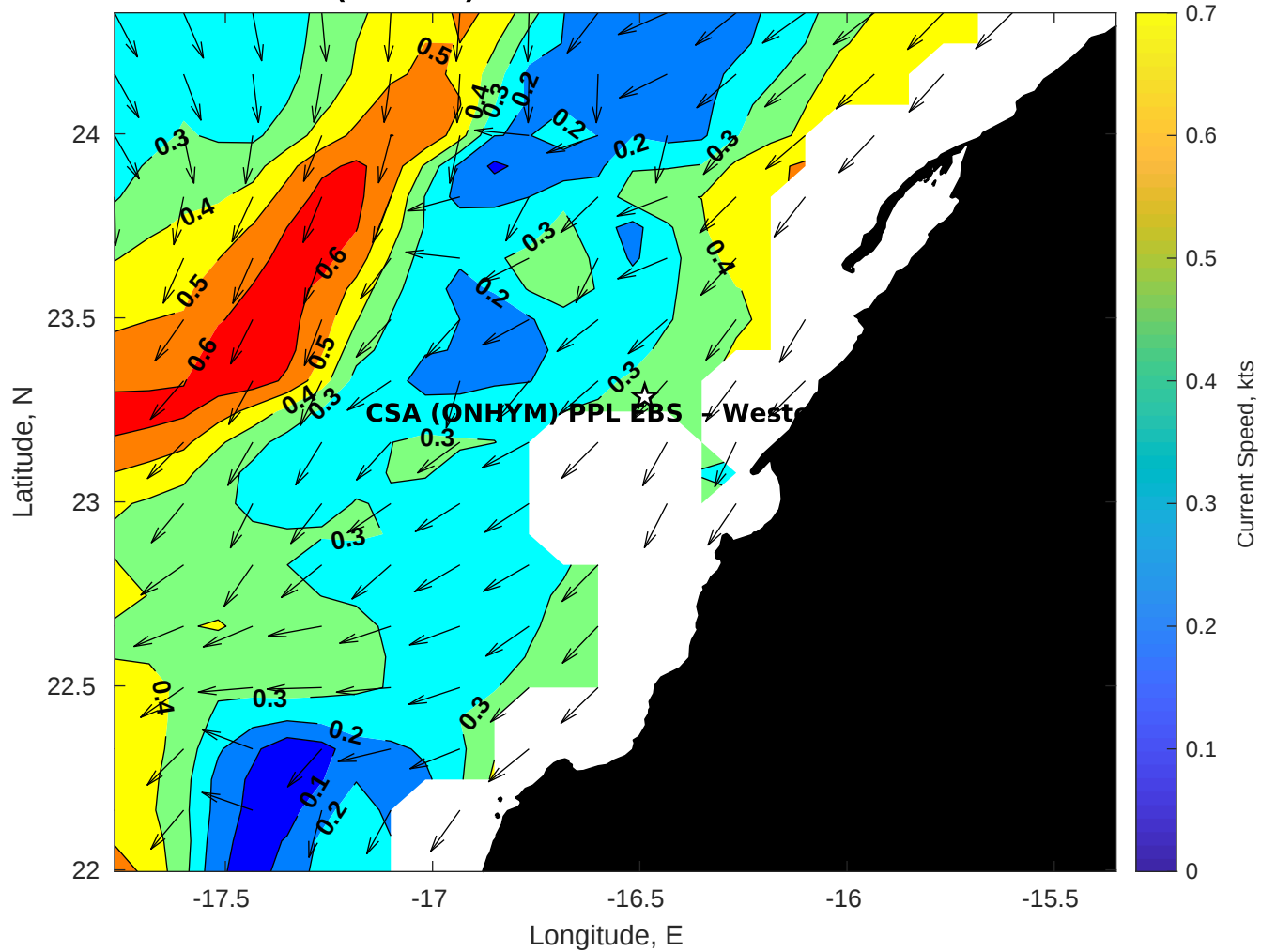
Surface Currents for CSA (ONHYM) PPL EBS - Western Sahara at 11-Oct-2025 00:00:00
