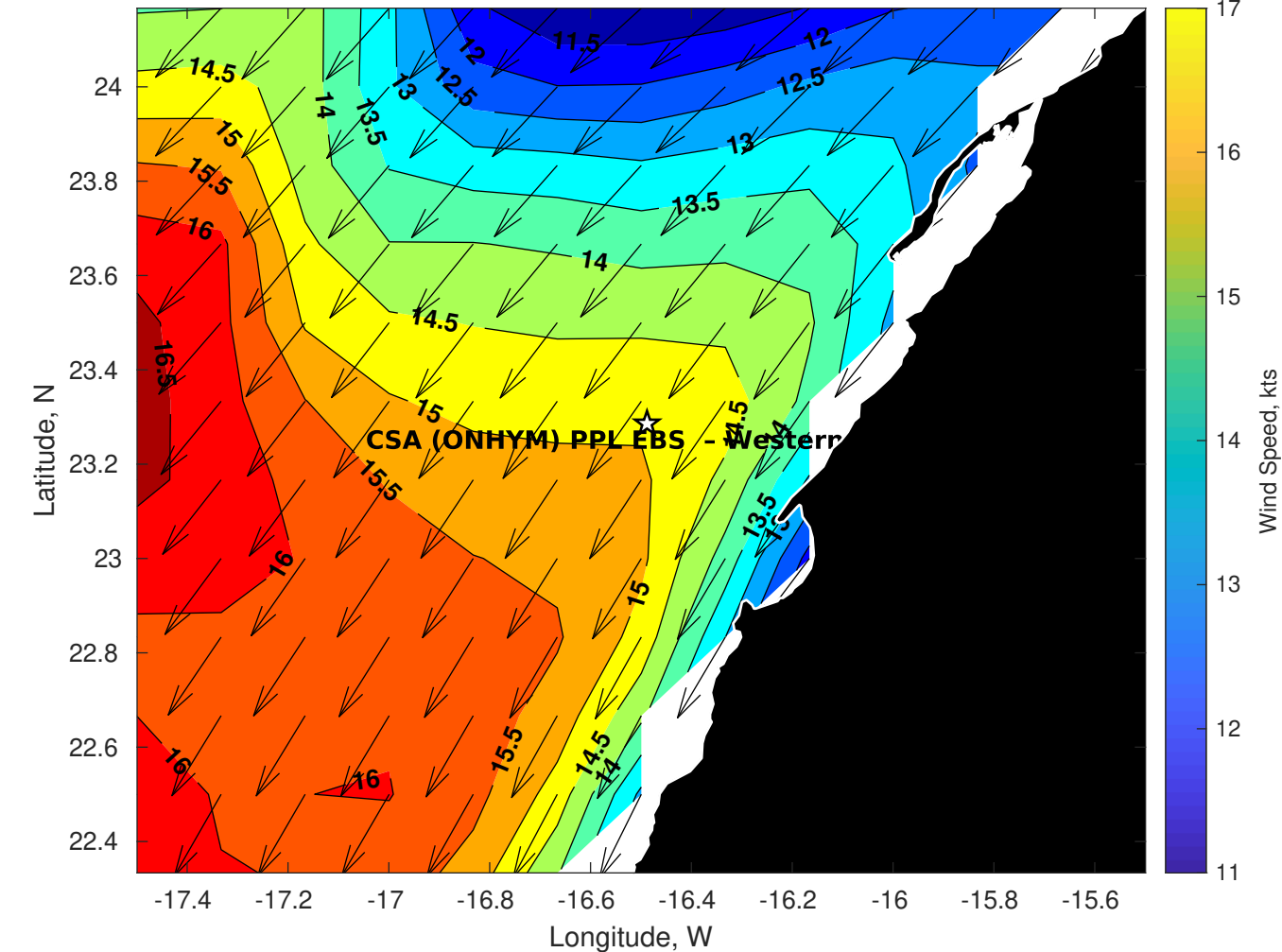
Winds (kts) for CSA (ONHYM) PPL EBS - Western Sahara at 12-Oct-2025 09:00:00
