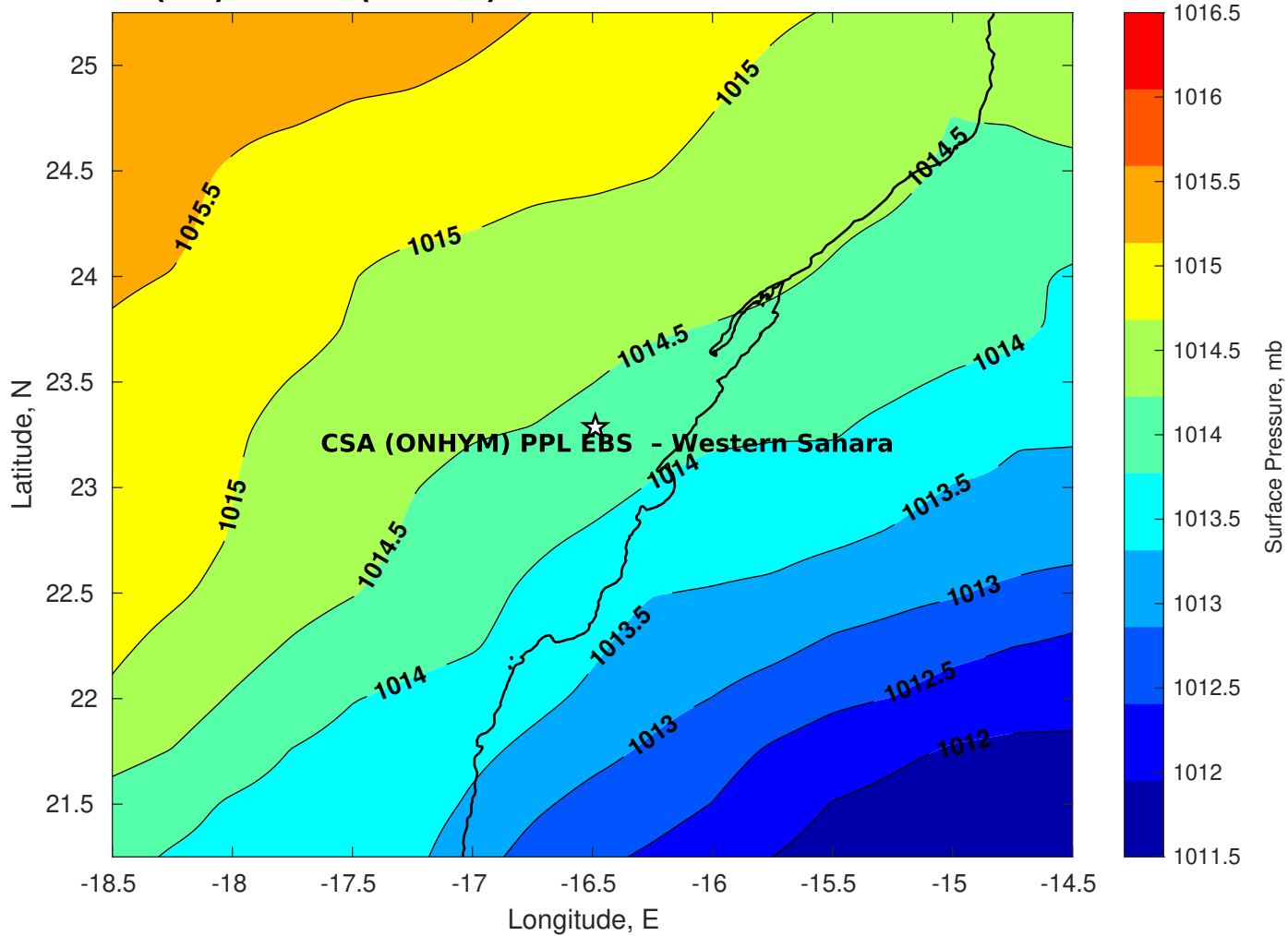
Surface Pressure (mb) for CSA (ONHYM) PPL EBS - Western Sahara at 13-Oct-2025 00:00:00
