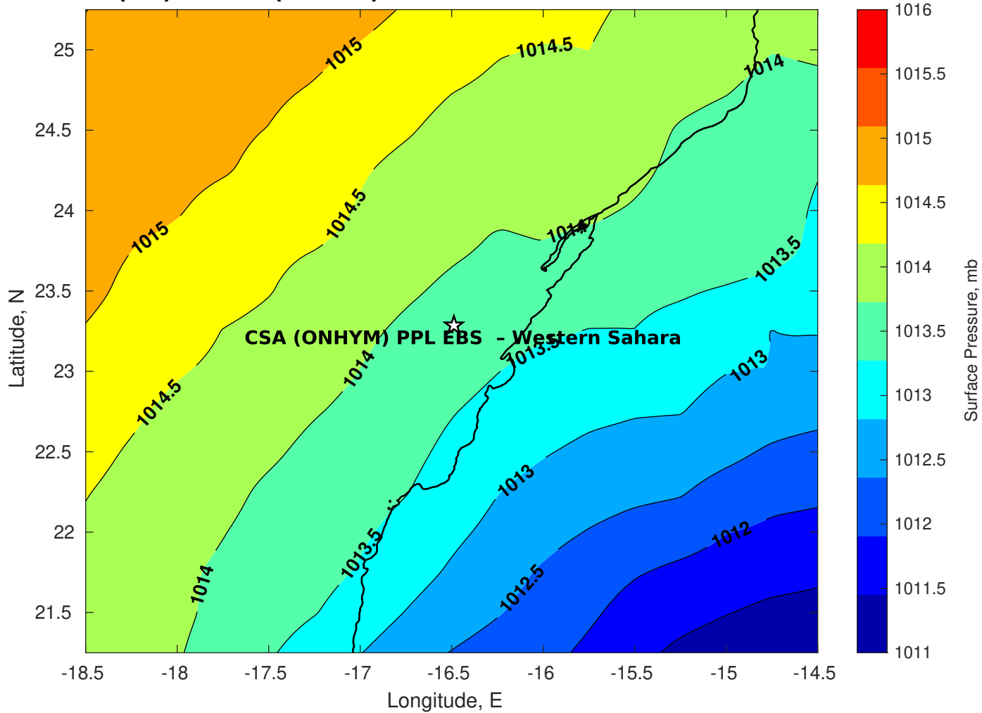
Surface Pressure (mb) for CSA (ONHYM) PPL EBS - Western Sahara at 14-Oct-2025 00:00:00
