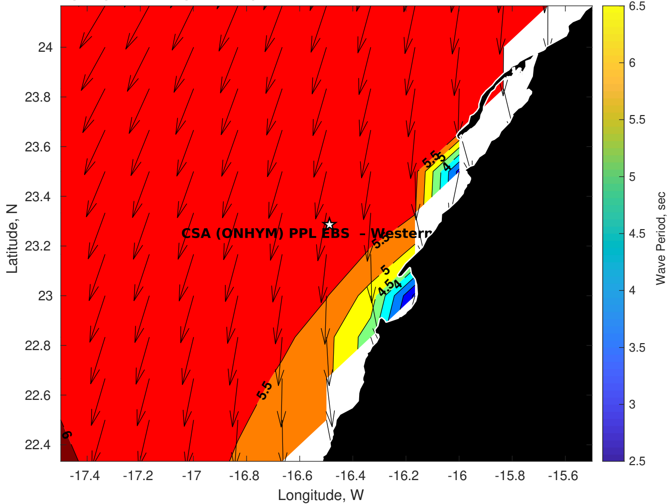
Wave Period (sec) for CSA (ONHYM) PPL EBS - Western Sahara at 12-Oct-2025 09:00:00
