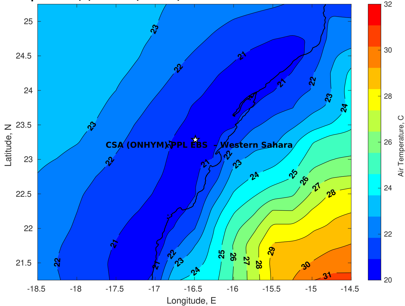
Air Temperature (C) for CSA (ONHYM) PPL EBS - Western Sahara at 12-Oct-2025
