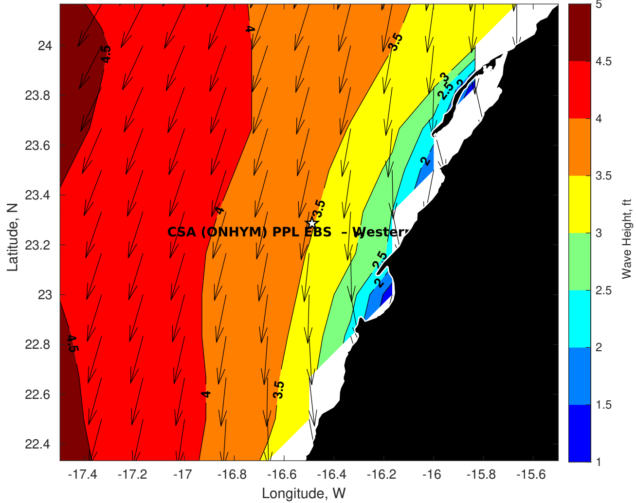
Wave Height (ft) for CSA (ONHYM) PPL EBS - Western Sahara at 12-Oct-2025 09:00:00
