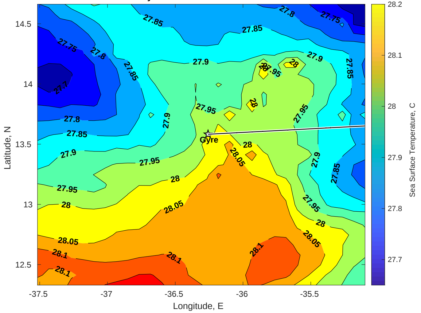
SST for Gyre at 11-Oct-2025 00:00:00
