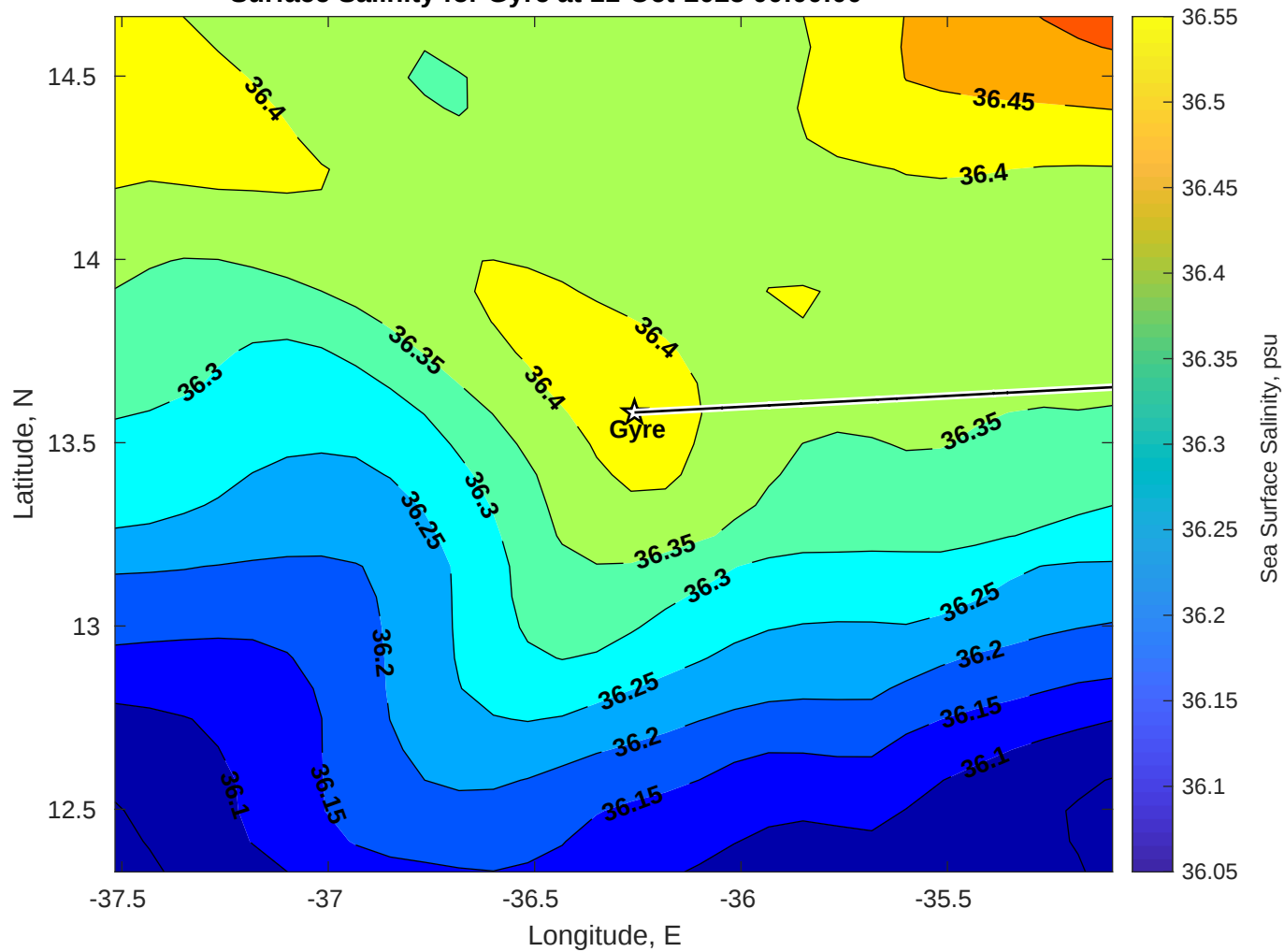
Surface Salinity for Gyre at 11-Oct-2025 00:00:00
