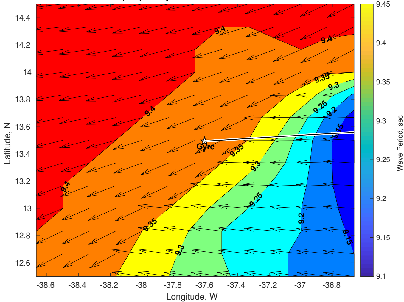
Wave Period (sec) for Gyre at 12-Oct-2025 09:00:00
