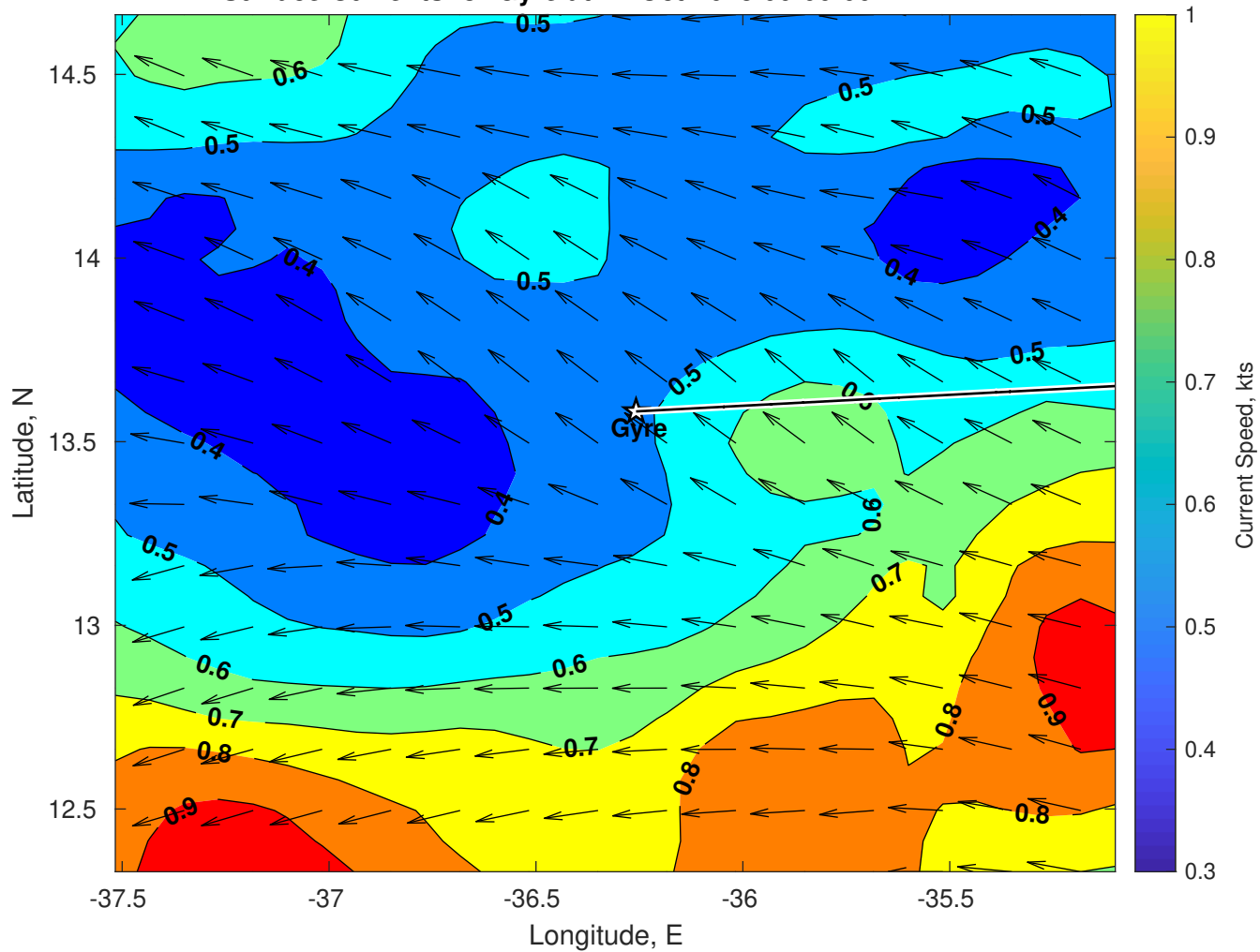
Surface Currents for Gyre at 11-Oct-2025 00:00:00
