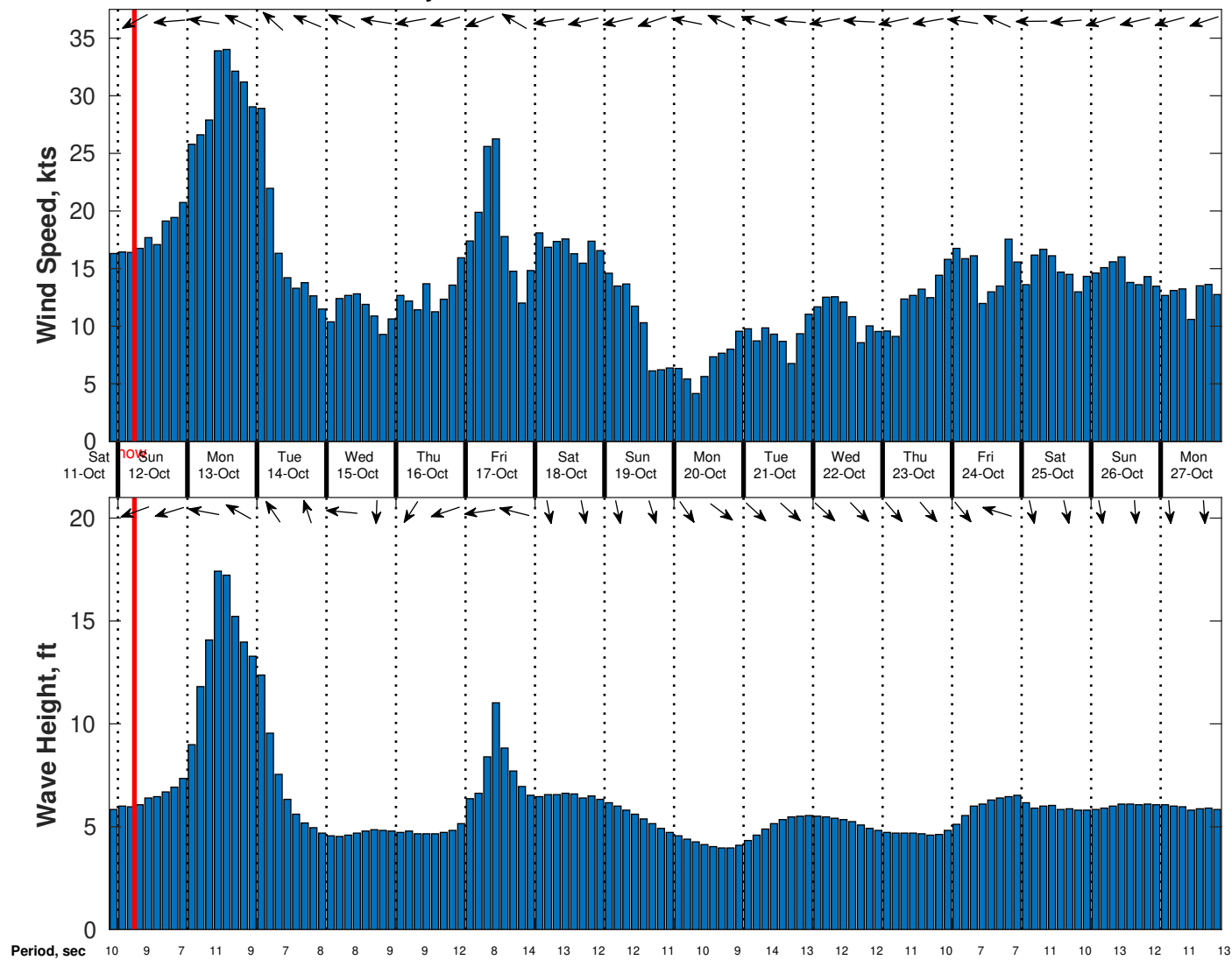
Wind & Wave Forecast for Gyre from 11-Oct-2025 21:00:00 to 27-Oct-2025 21:00:00
