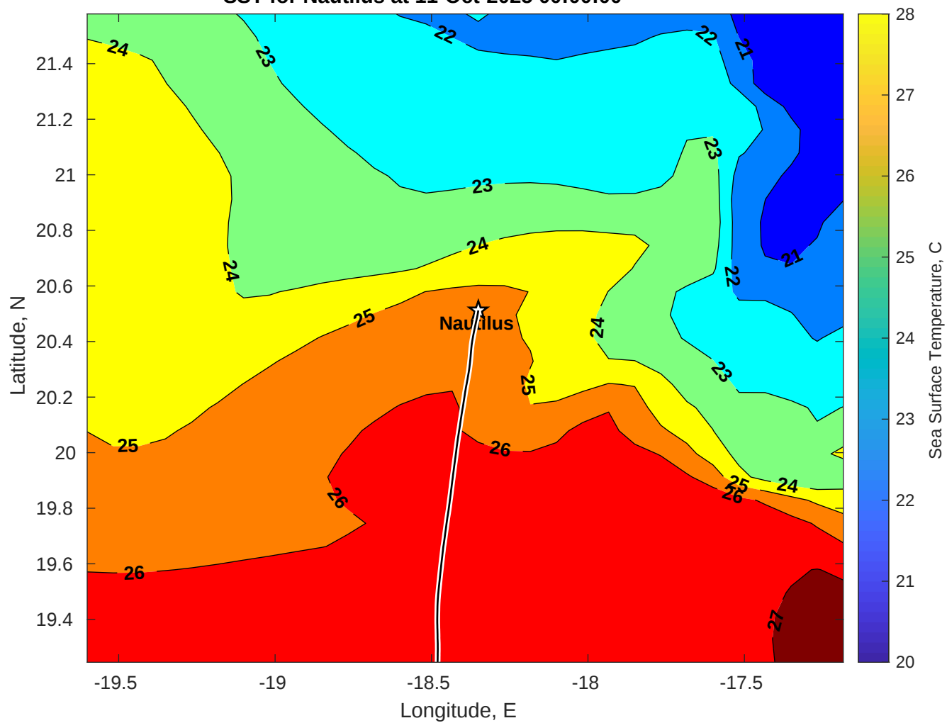
SST for Nautilus at 11-Oct-2025 00:00:00
