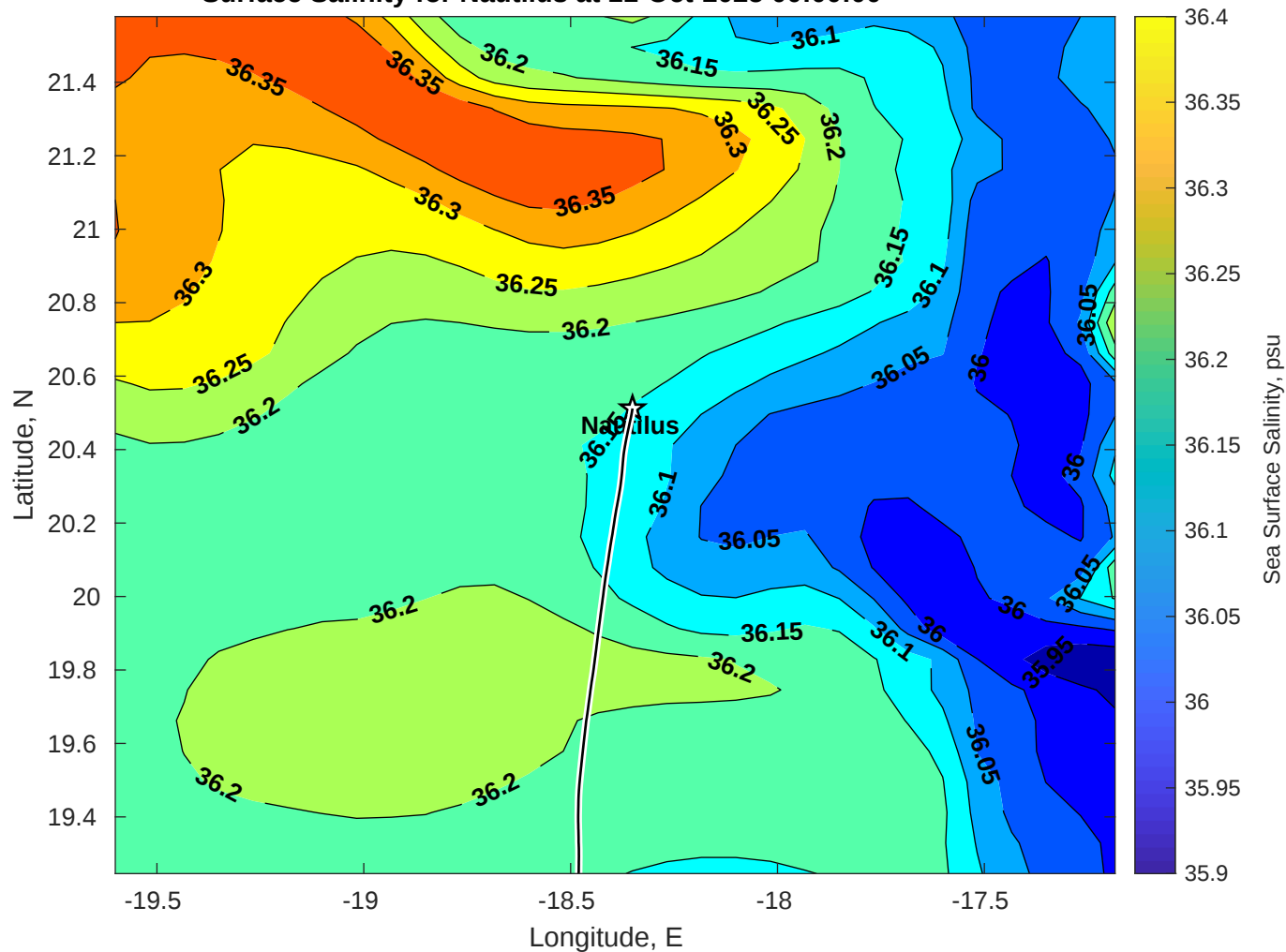
Surface Salinity for Nautilus at 11-Oct-2025 00:00:00
