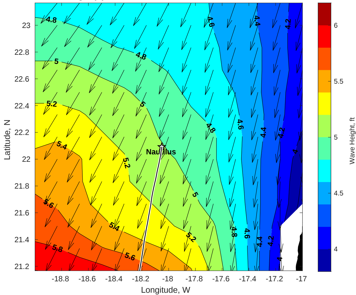
Wave Height (ft) for Nautilus at 12-Oct-2025 09:00:00
