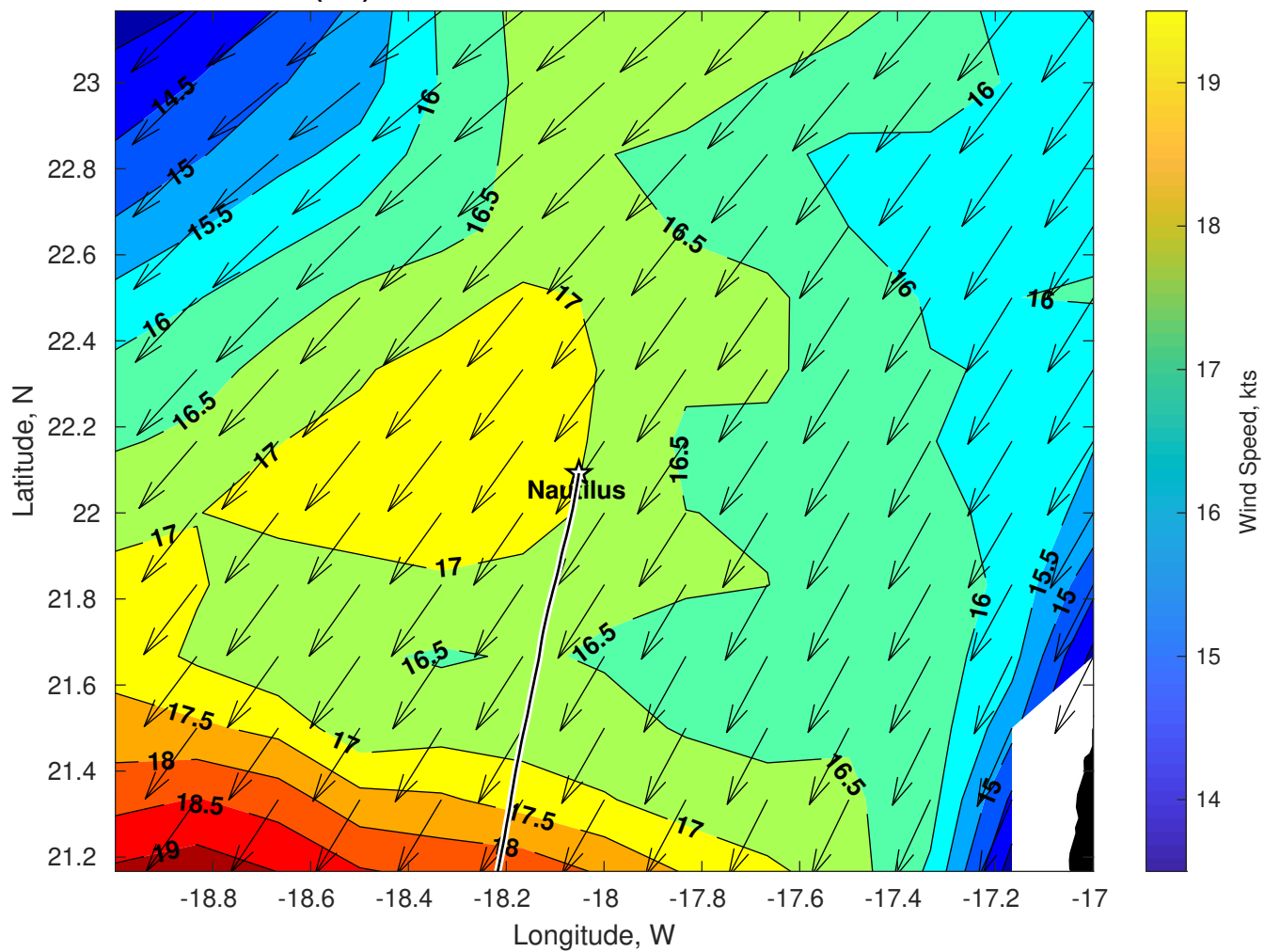
Winds (kts) for Nautilus at 12-Oct-2025 09:00:00
