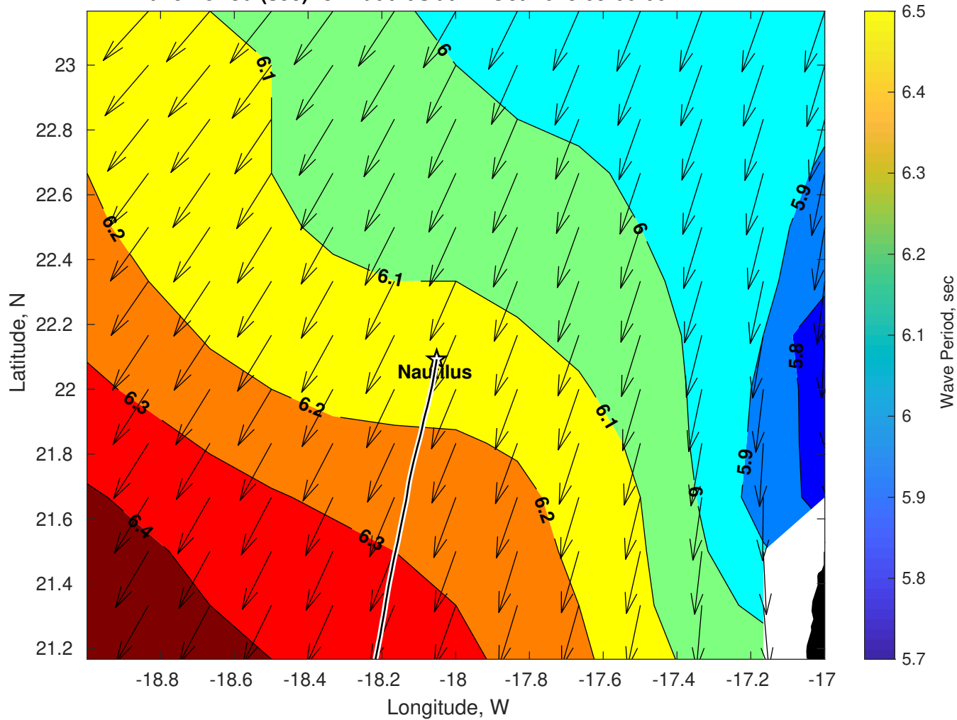
Wave Period (sec) for Nautilus at 12-Oct-2025 09:00:00
