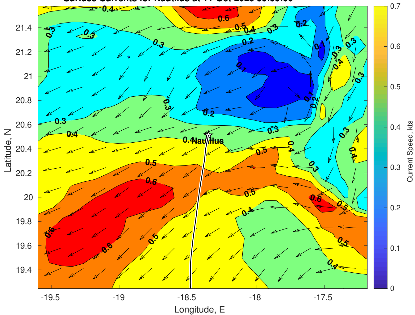
Surface Currents for Nautilus at 11-Oct-2025 00:00:00
