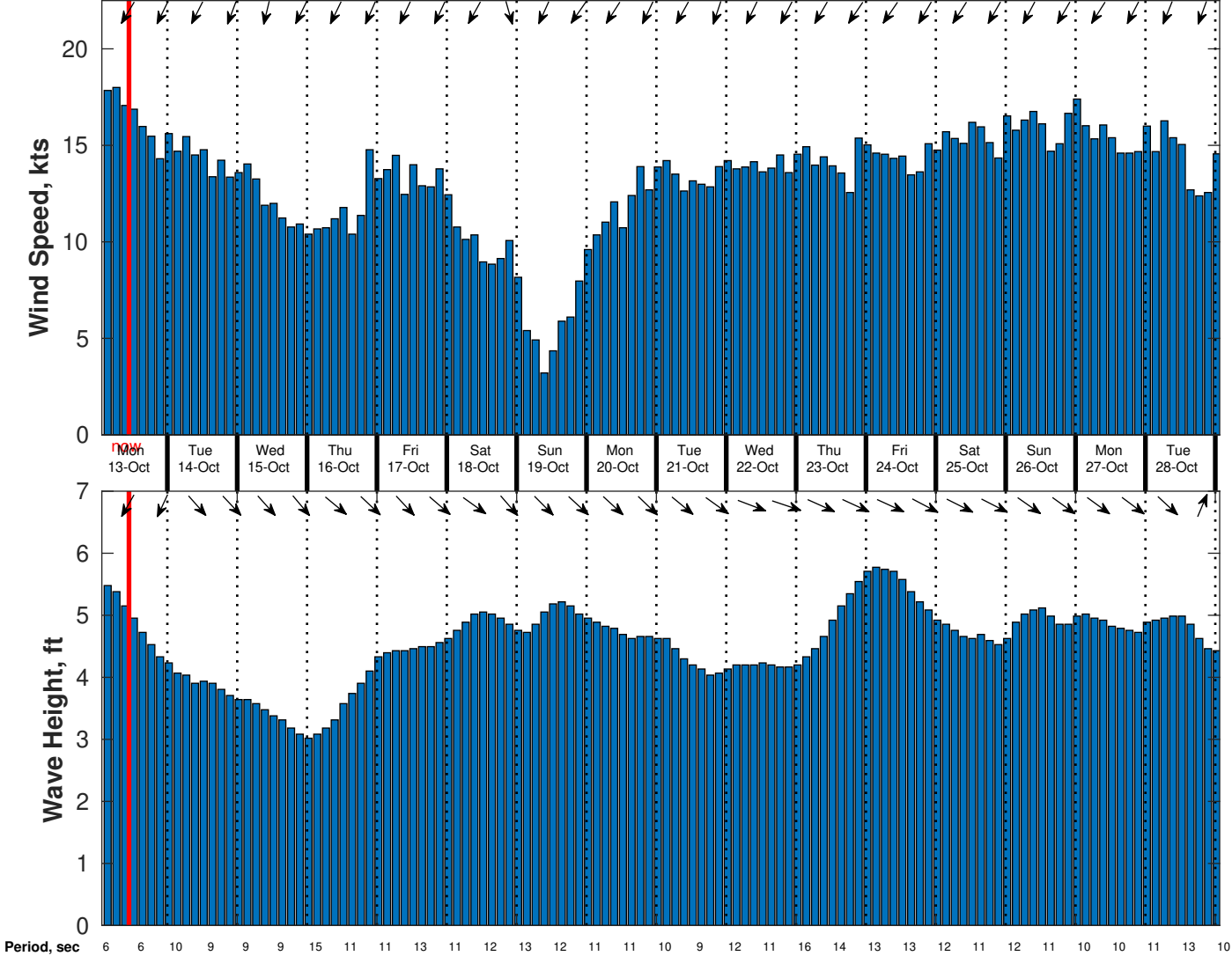
Wind & Wave Forecast for Nautilus from 12-Oct-2025 02:00:00 to 28-Oct-2025 02:00:00
