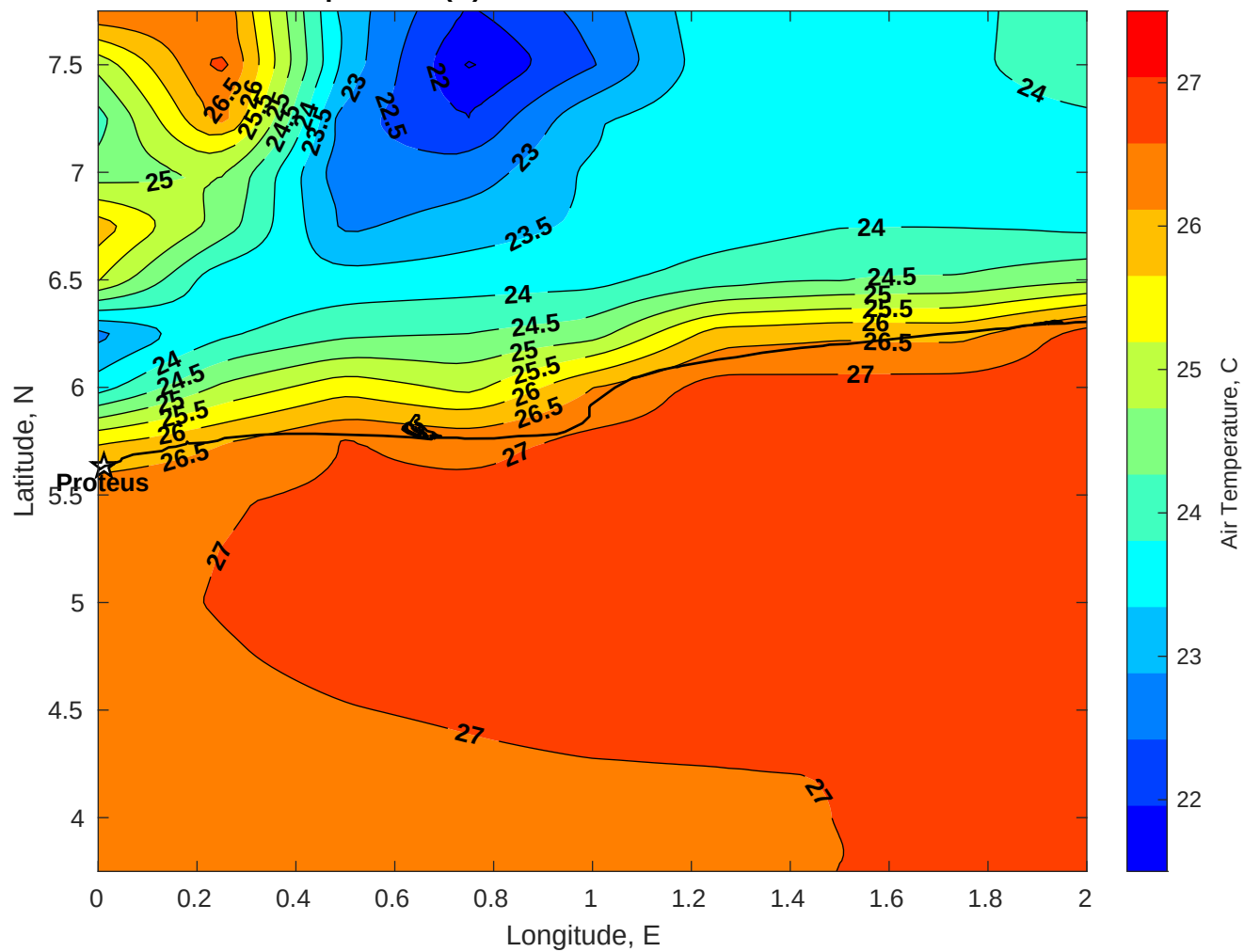
Air Temperature (C) for Proteus at 12-Oct-2025
