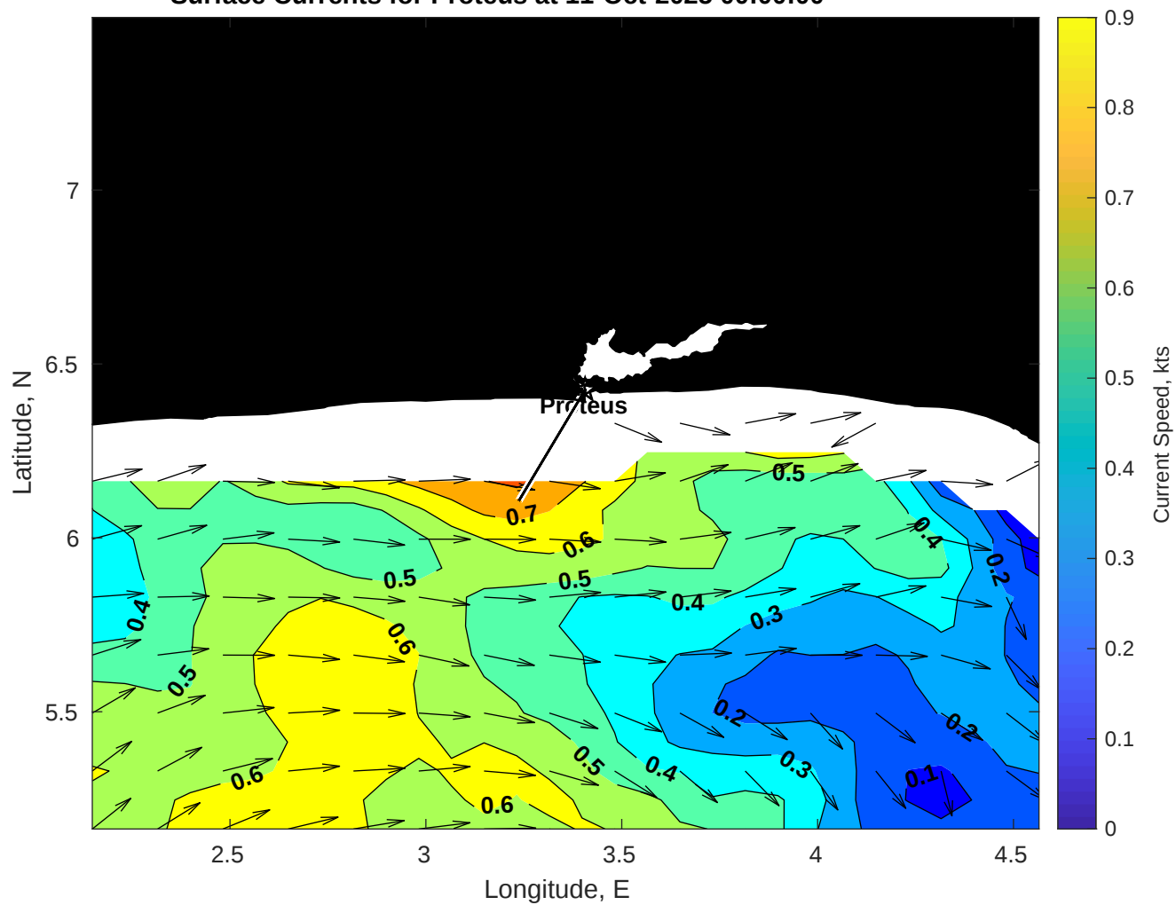
Surface Currents for Proteus at 11-Oct-2025 00:00:00
