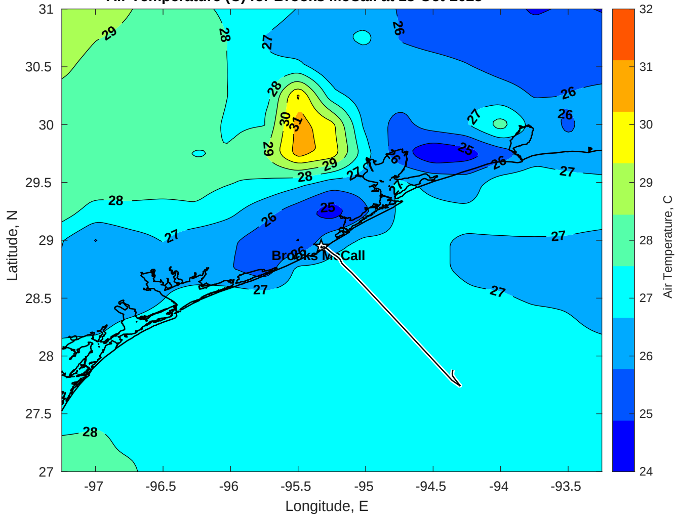
Air Temperature (C) for Brooks McCall at 13-Oct-2025
