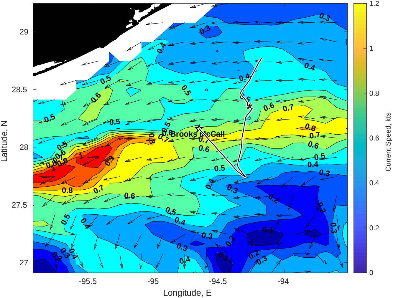
Surface Currents for Brooks McCall at 12-Oct-2025 00:00:00
