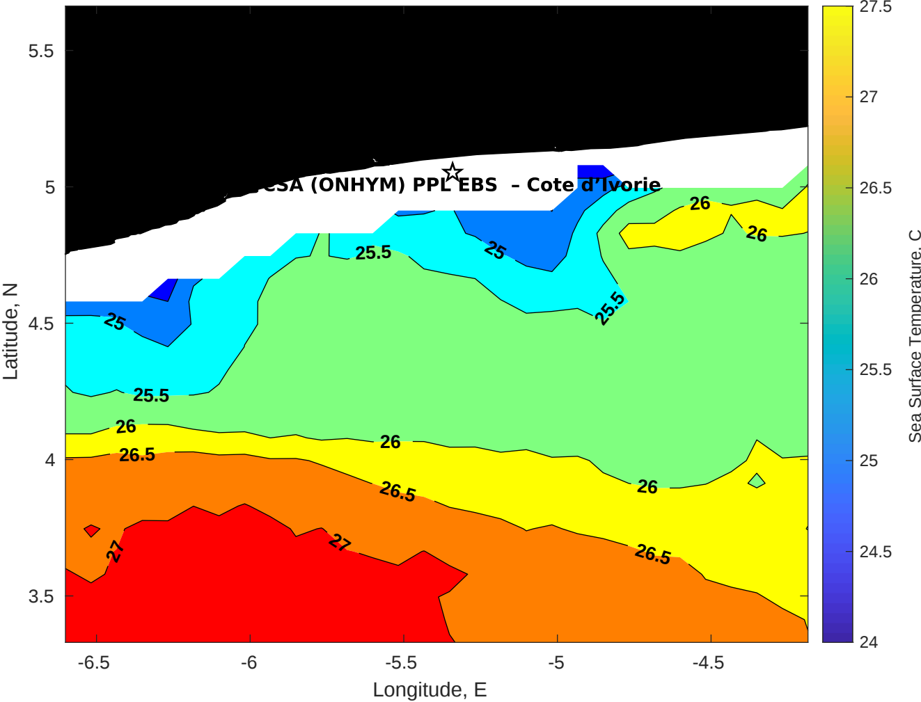
SST for CSA (ONHYM) PPL EBS - Cote d'Ivoire at 12-Oct-2025 00:00:00
