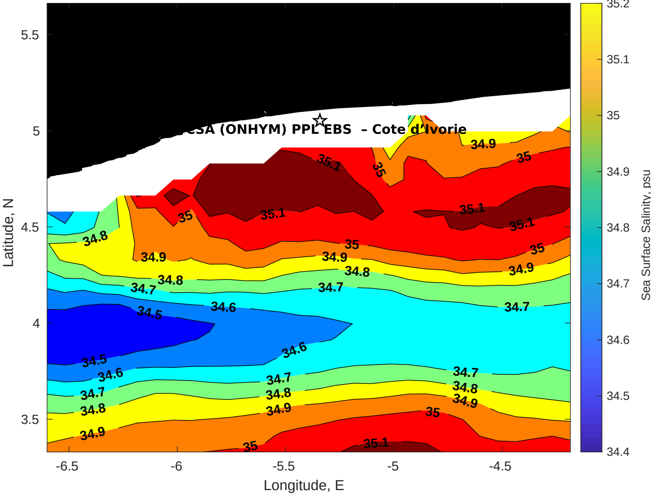
Surface Salinity for CSA (ONHYM) PPL EBS - Cote d'Ivoire at 12-Oct-2025 00:00:00
